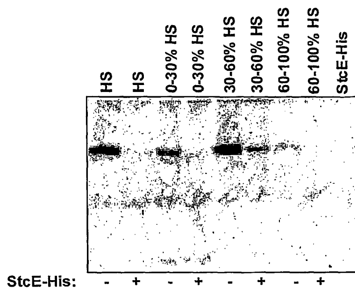
Figure 5. StcE-His cleaves C1 inhibitor in human serum.
