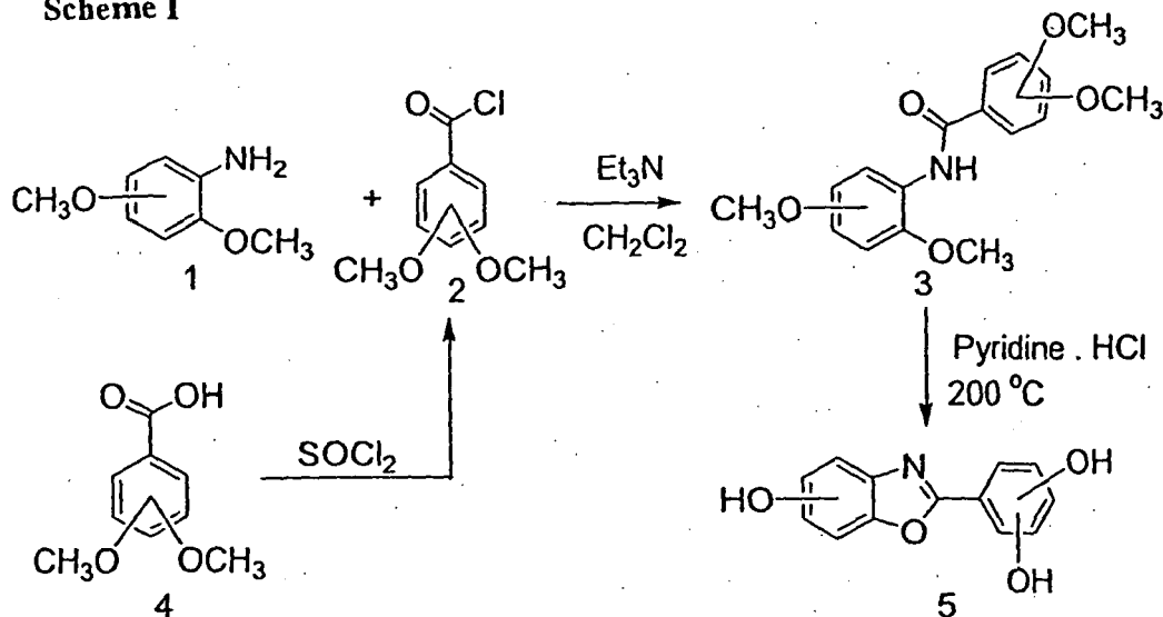
Scheme I
