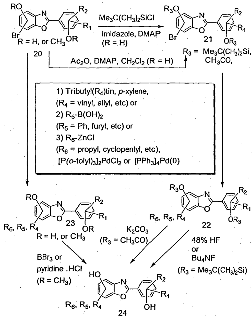
Scheme V
