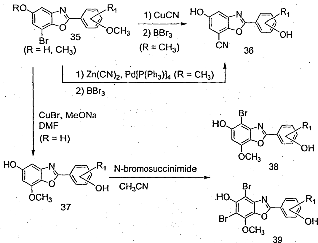
Scheme VIII
