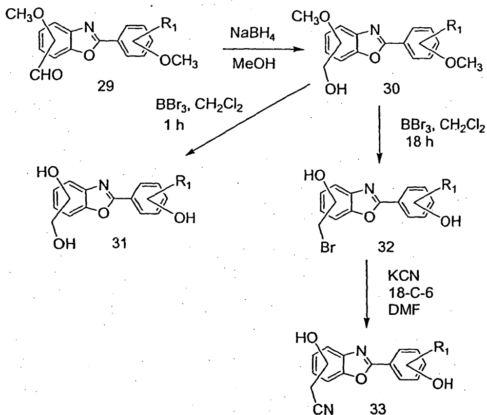
Scheme VII
