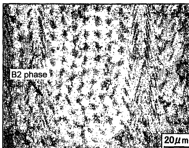
Metallic structure of Ir-1.5Al-10.5W alloy
