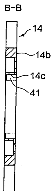
cross section
