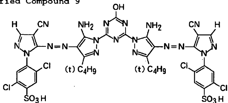
Exemplified Compound 9
