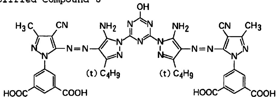
Exemplified Compound 6
