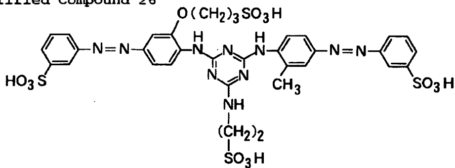
Exemplified Compound 26
