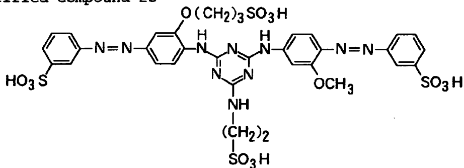
Exemplified Compound 25
