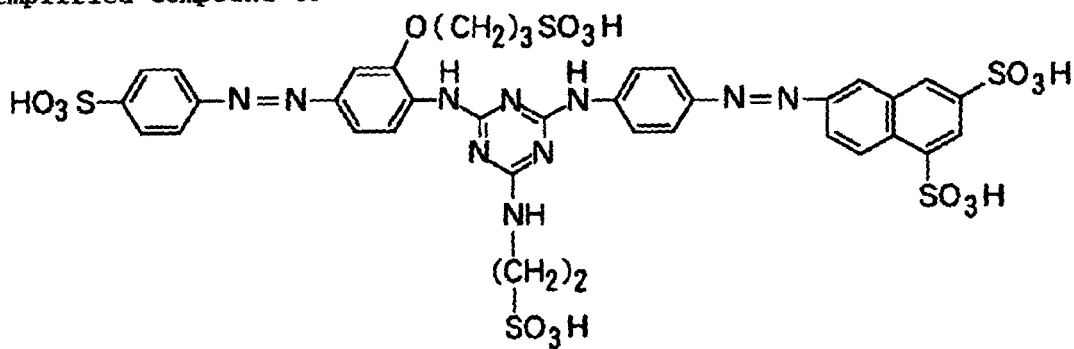
Exemplified Compound 40
