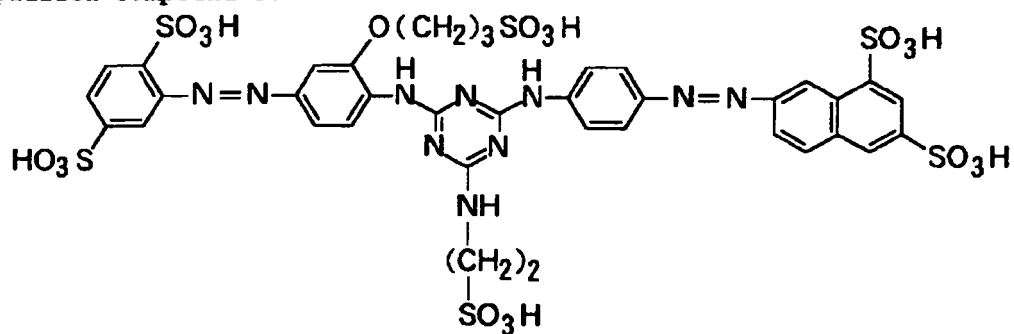
Exemplified Compound 38
