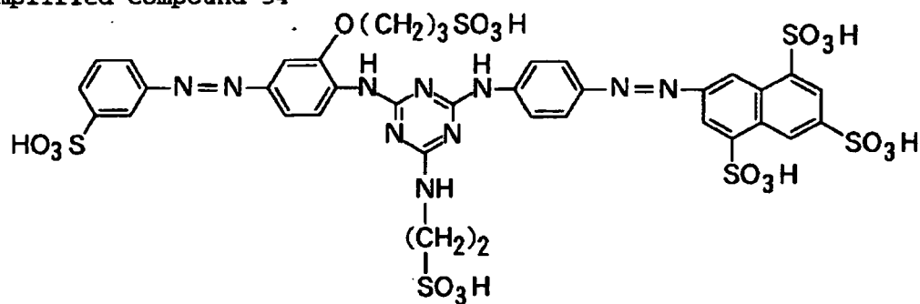
Exemplified Compound 34
