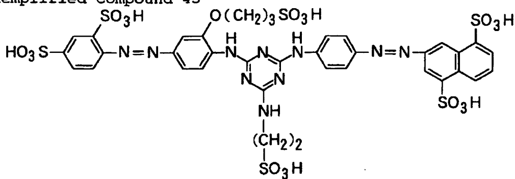
Exemplified Compound 45
