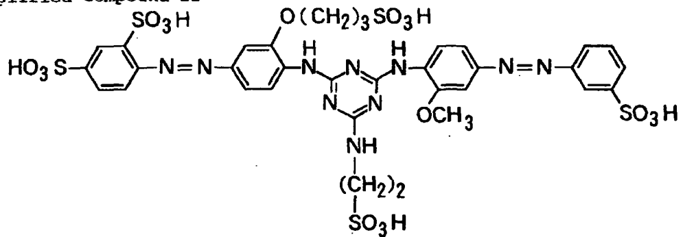
Exemplified Compound 22
