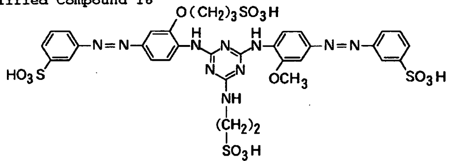
Exemplified Compound 16
