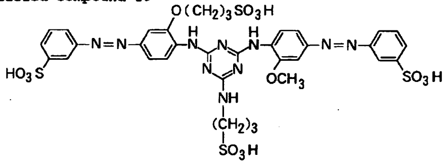
Exemplified Compound 19
