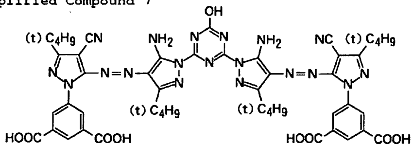
Exemplified Compound 7
