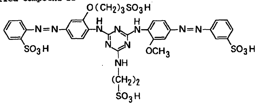
Exemplified Compound 21
