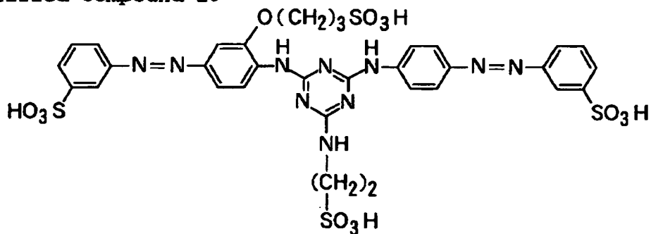
Exemplified Compound 29
