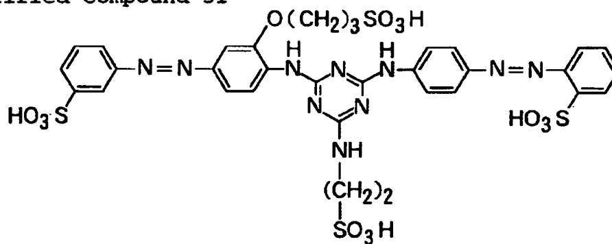
Exemplified Compound 31
