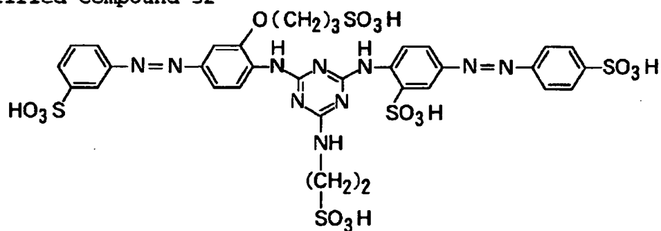
Exemplified Compound 32
