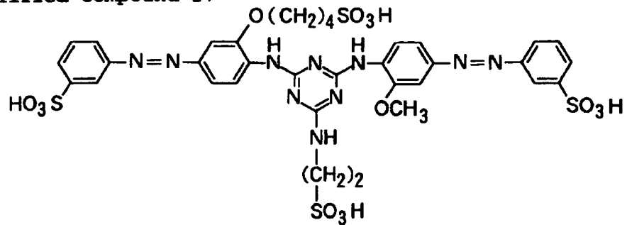
Exemplified Compound 17
