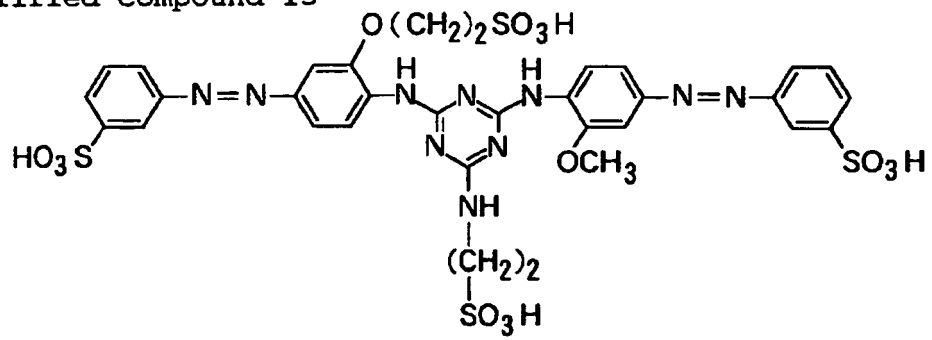
Exemplified Compound 15
