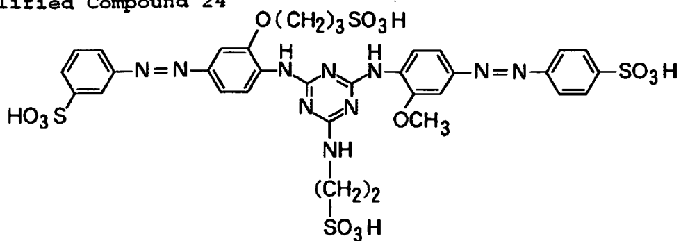
Exemplified Compound 24
