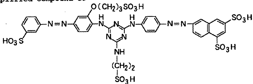
Exemplified Compound 39
