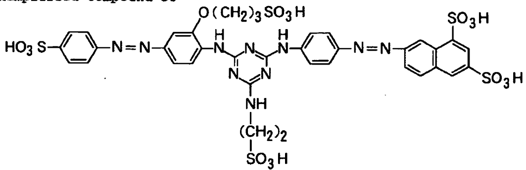
Exemplified Compound 36
