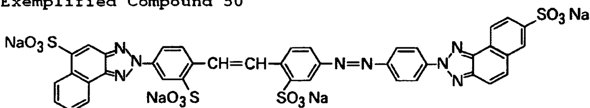
Exemplified Compound 50
