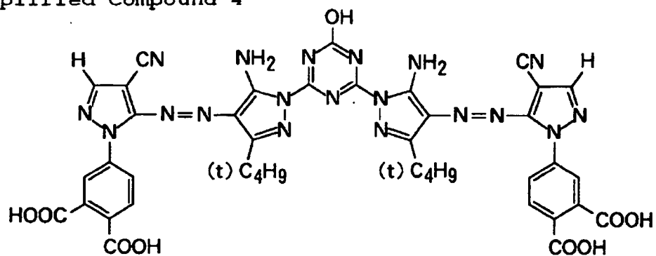
Exemplified Compound 4
