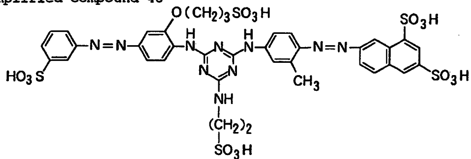
Exemplified Compound 48
