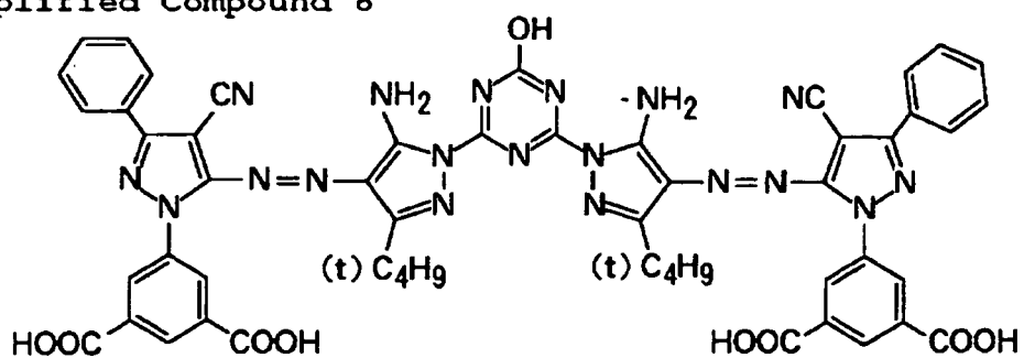
Exemplified Compound 8
