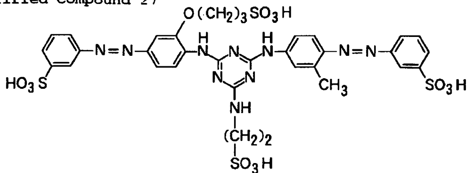
Exemplified Compound 27
