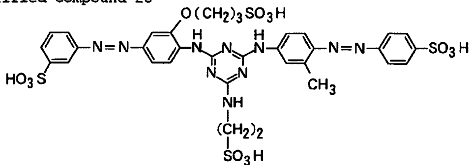
Exemplified Compound 28
