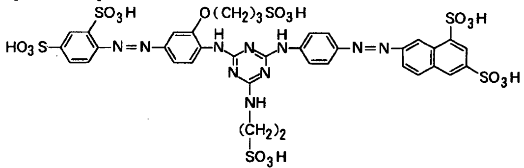
Exemplified Compound 37
