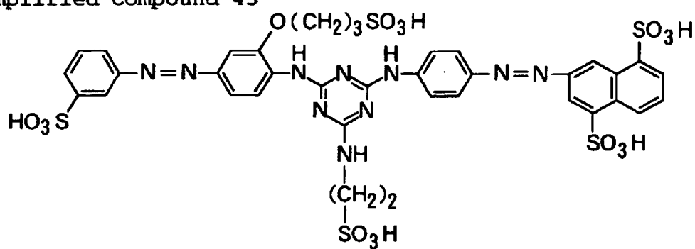
Exemplified Compound 43
