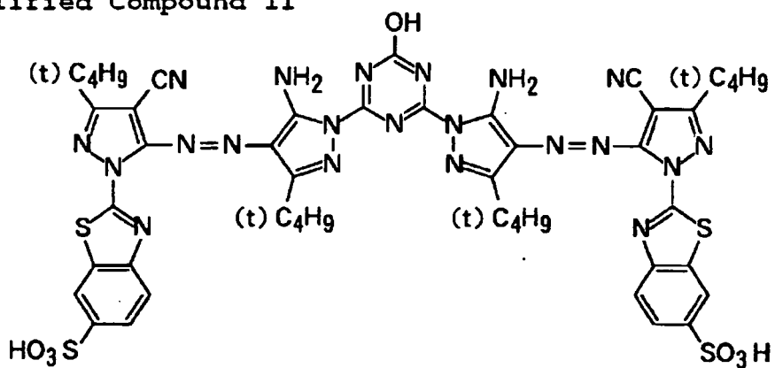
Exemplified Compound 11
