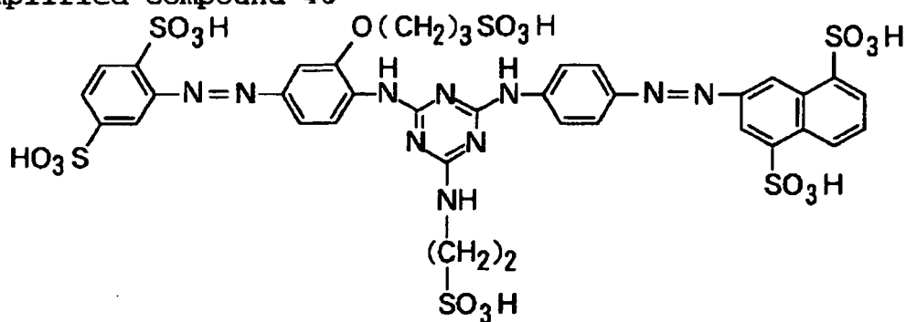
Exemplified Compound 46
