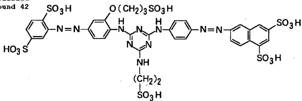
Exemplified Compound 43
