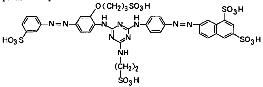
Exemplified Compound 35
