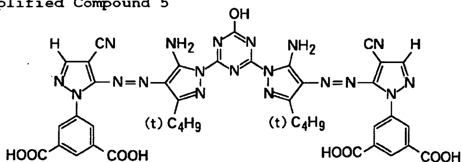
Exemplified Compound 5
