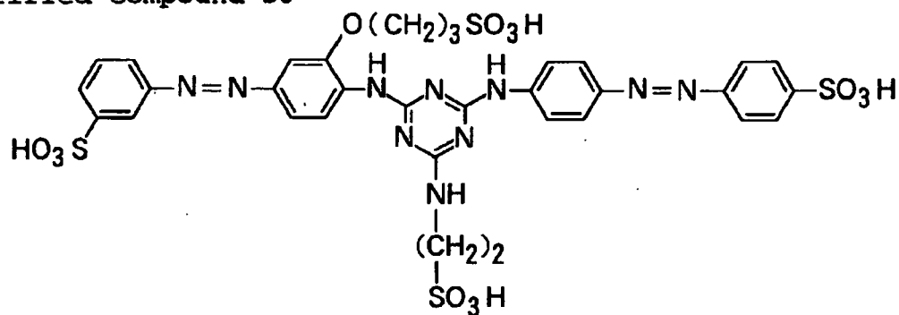
Exemplified Compound 30
