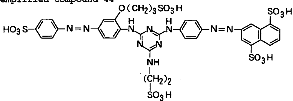
Exemplified Compound 44
