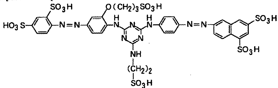
Exemplified Compound 41
