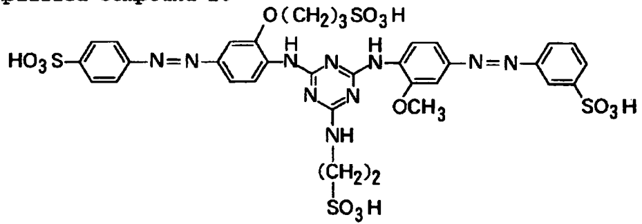
Exemplified Compound 20
