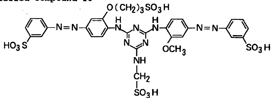
Exemplified Compound 18
