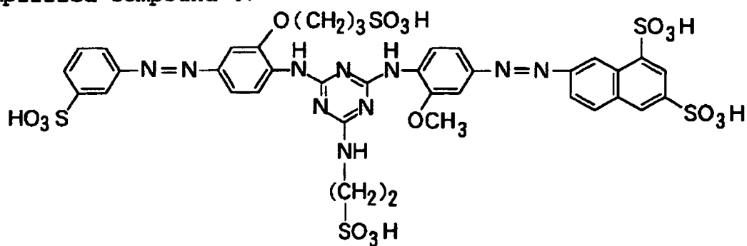
Exemplified Compound 47
