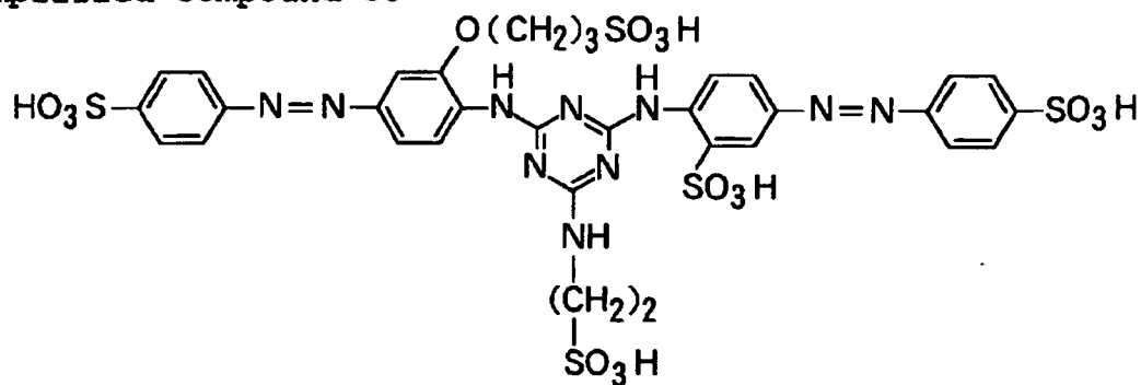
Exemplified Compound 33
