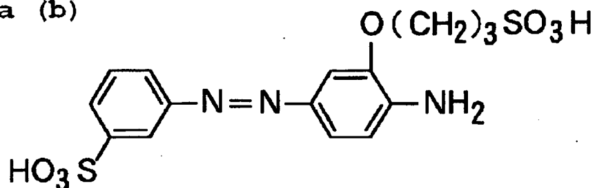
Formula (b)
