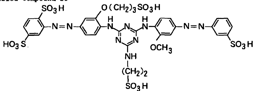
Exemplified Compound 23
