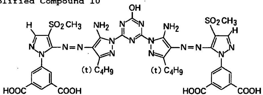
Exemplified Compound 10
