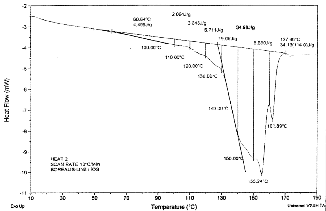
Figure 6: SIST Curve E 3 (8,27 mg sample)
