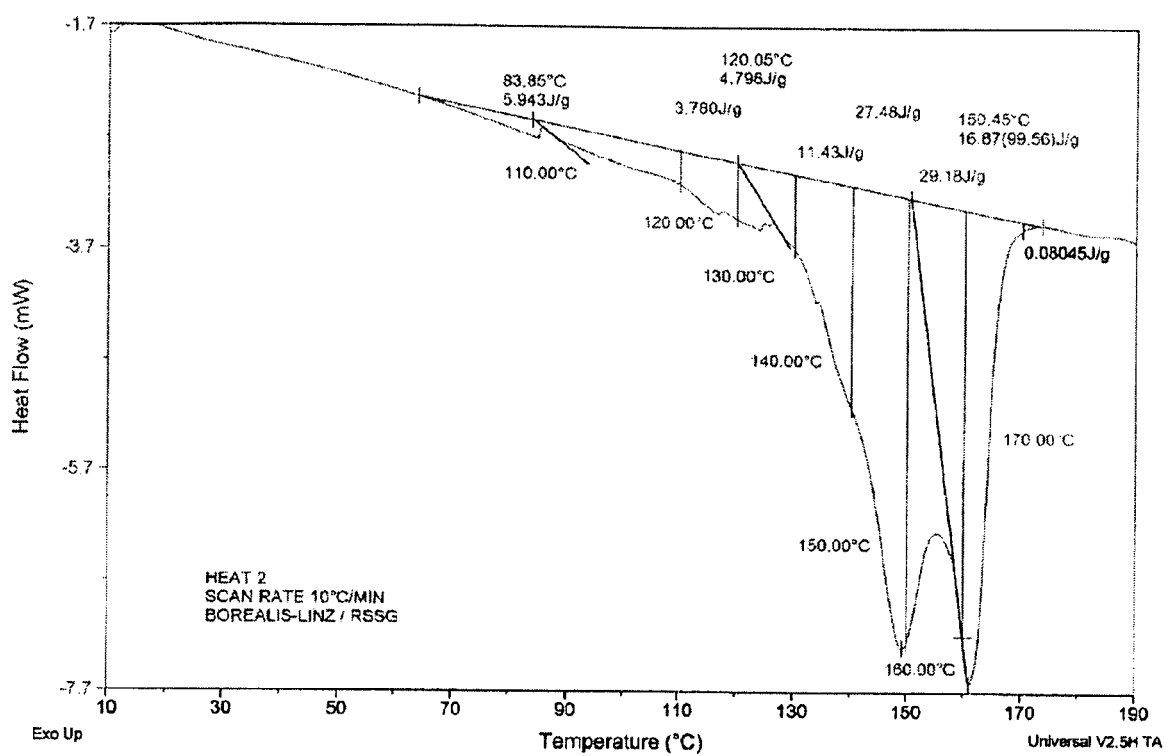
Figure 3: SIST Curve E 1 (6,76 mg sample)
