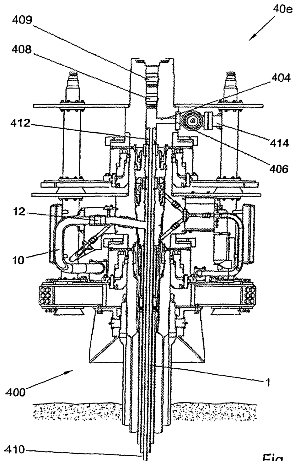
TYPICAL SECTION
