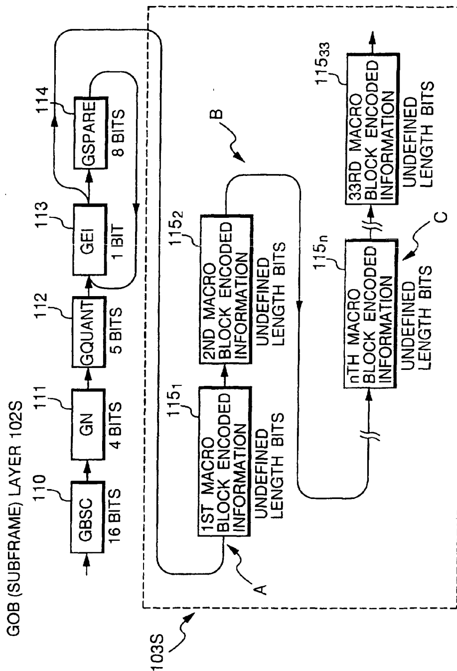
FIG. 3 PRIOR ART
