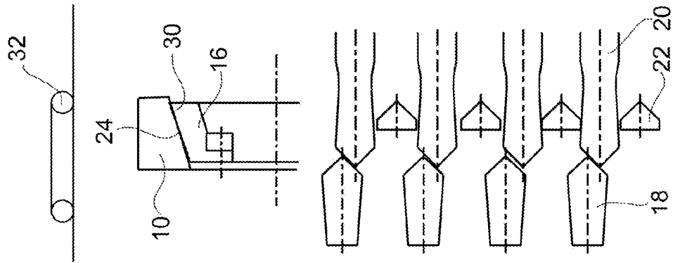
FIG.4C ( PRIOR ART )
