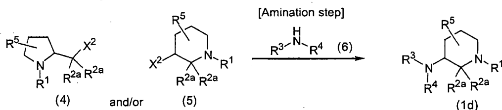
[Reaction schema 3]
