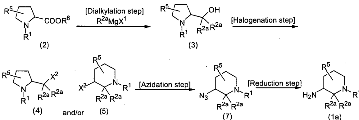
[Reaction schema 2]
