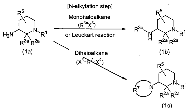
[Reaction schema 3]
