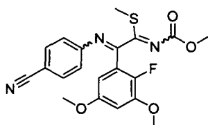
[Chemical Formula 44]
