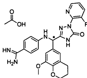
[Chemical Formula 146]
