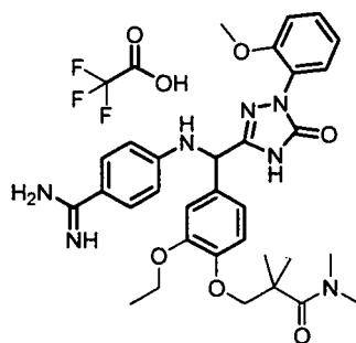
[Chemical Formula 753]
