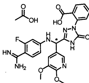
[Chemical Formula 801]
