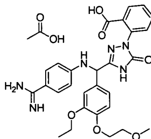
[Chemical Formula 721]
