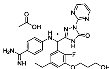
[Chemical Formula 783]
