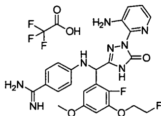
[Chemical Formula 359]
