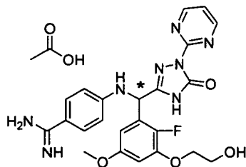
[Chemical Formula 439]
