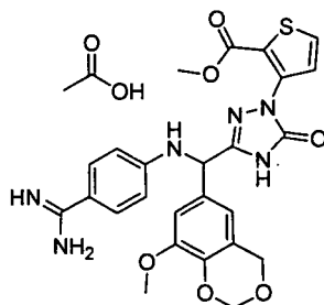
[Chemical Formula 388]
