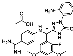
[Chemical Formula 787]
