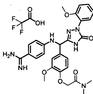
[Chemical Formula 756]
