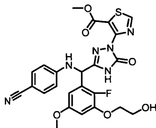
[Chemical Formula 472]
