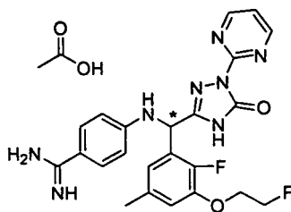
[Chemical Formula 622]
