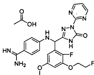
[Chemical Formula 56]
