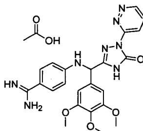
[Chemical Formula 269]
