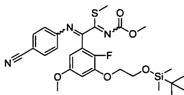
[Chemical Formula 467]
