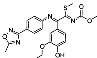
[Chemical Formula 328]
