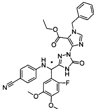
[Chemical Formula 486]
