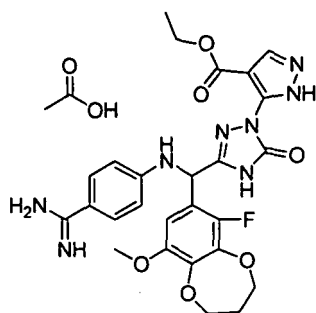
[Chemical Formula 504]
