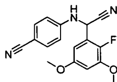
[Chemical Formula 40]
