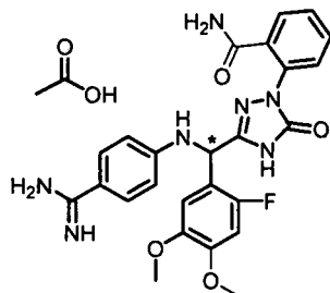
[Chemical Formula 302]
