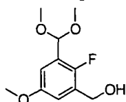
[Chemical Formula 547]
