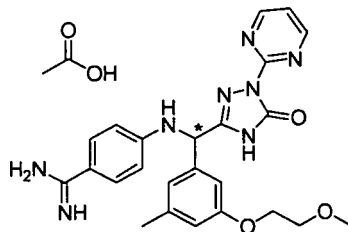
[Chemical Formula 277]
