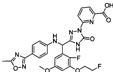
[Chemical Formula 443]
