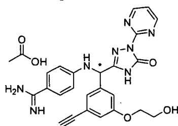
[Chemical Formula 543]
