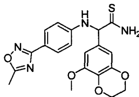
[Chemical Formula 114]
