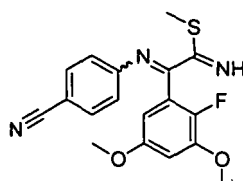
[Chemical Formula 43]
