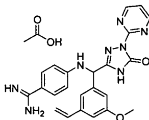
[Chemical Formula 710]
