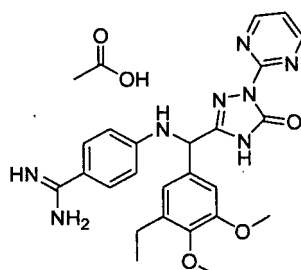
[Chemical Formula 600]
