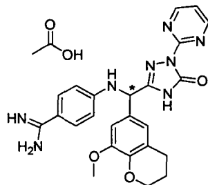
[Chemical Formula 133]
