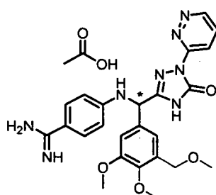
[Chemical Formula 656]
