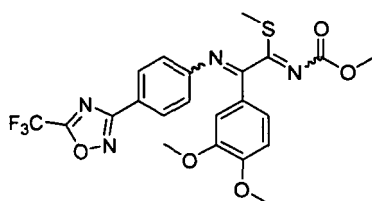
[Chemical Formula 505]
