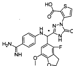
[Chemical Formula 546]
