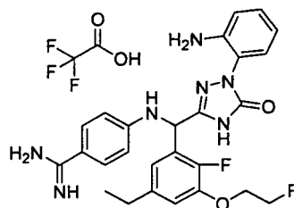
[Chemical Formula 696]
