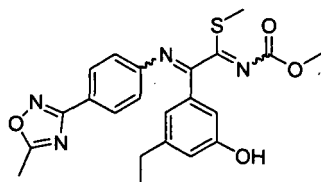
[Chemical Formula 241]
