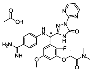
[Chemical Formula 90]
