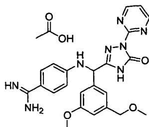
[Chemical Formula 74]
