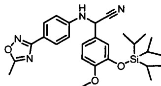
[Chemical Formula 94]
