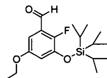
[Chemical Formula 230]
