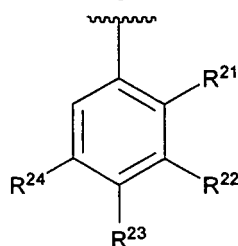
[Chemical Formula 15]
