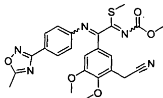
[Chemical Formula 137]
