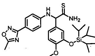
[Chemical Formula 95]
