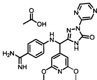
[Chemical Formula 660]
