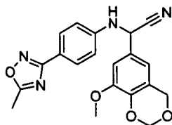
[Chemical Formula 119]
