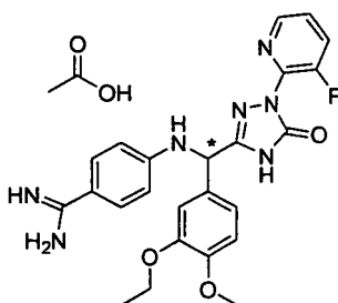
[Chemical Formula 345]
