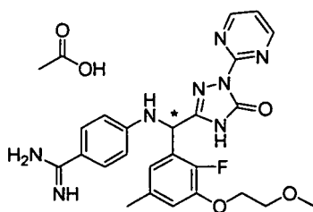
[Chemical Formula 735]
