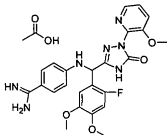
[Chemical Formula 326]
