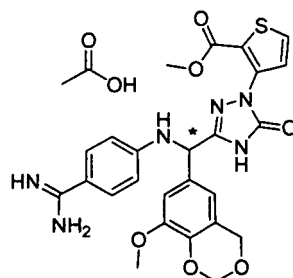
[Chemical Formula 389]
