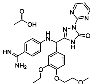
[Chemical Formula 724]
