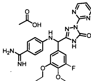
[Chemical Formula 645]
