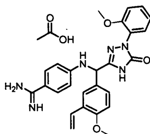
[Chemical Formula 739]
