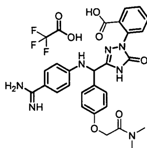
[Chemical Formula 745]
