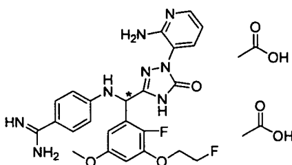
[Chemical Formula 205]
