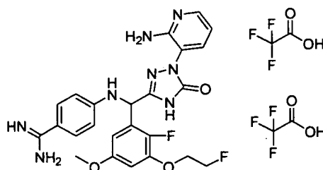
[Chemical Formula 204]
