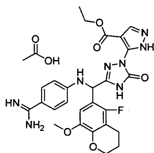
[Chemical Formula 778]
