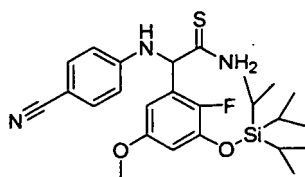
[Chemical Formula 414]
