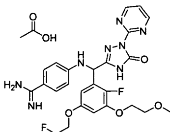
[Chemical Formula 623]
