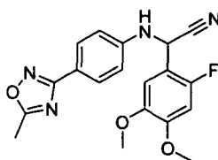
[Chemical Formula 32]
