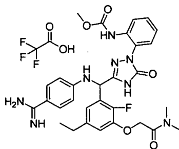
[Chemical Formula 357]
