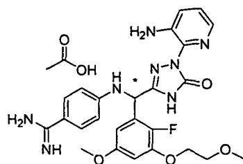
[Chemical Formula 532]
