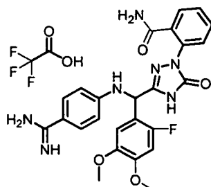
[Chemical Formula 301]
