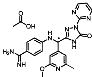
[Chemical Formula 177]
