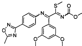
[Chemical Formula 567]
