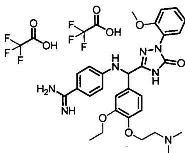
[Chemical Formula 761]
