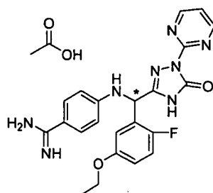
[Chemical Formula 280]
