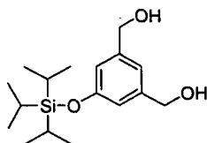
[Chemical Formula 77]
