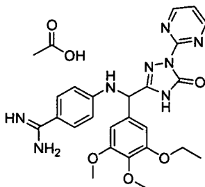
[Chemical Formula 614]
