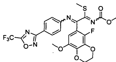
[Chemical Formula 490]
