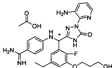
[Chemical Formula 535]
