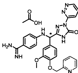
[Chemical Formula 754]
