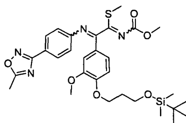
[Chemical Formula 536]
