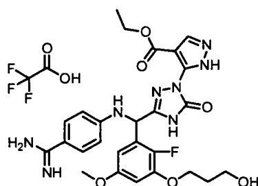
[Chemical Formula 455]
