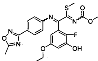
[Chemical Formula 231]
