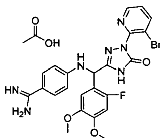
[Chemical Formula 347]
