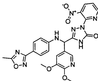
[Chemical Formula 482]
