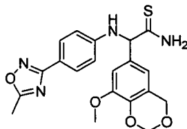
[Chemical Formula 120]
