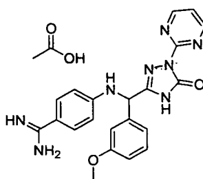
[Chemical Formula 707]
