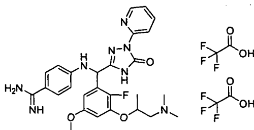
[Chemical Formula 85]
