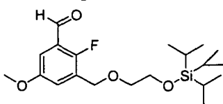
[Chemical Formula 550]
