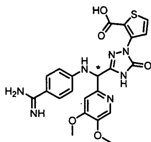
[Chemical Formula 435]
