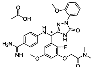
[Chemical Formula 619]
