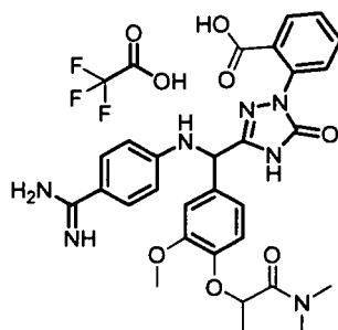
[Chemical Formula 748]
