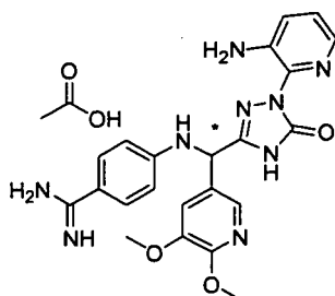
[Chemical Formula 483]
