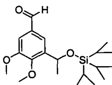
[Chemical Formula 134]
