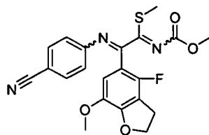
[Chemical Formula 408]
