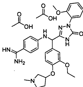
[Chemical Formula 718]
