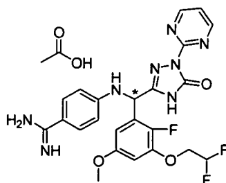
[Chemical Formula 288]
