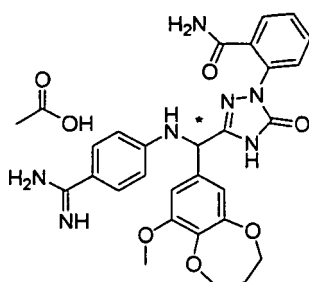
[Chemical Formula 545]
