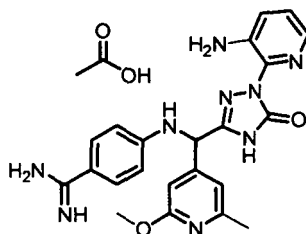
[Chemical Formula 112]
