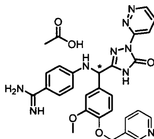
[Chemical Formula 760]
