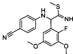
[Chemical Formula 42]
