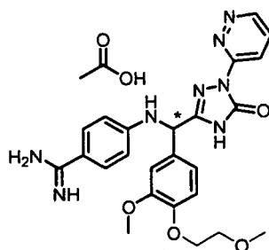
[Chemical Formula 757]
