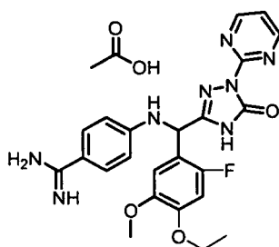
[Chemical Formula 740]
