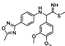
[Chemical Formula 169]
