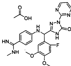
[Chemical Formula 202]
