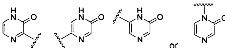
[Chemical Formula 14]
