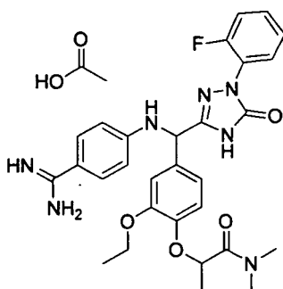
[Chemical Formula 719]
