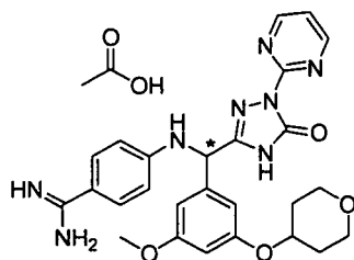
[Chemical Formula 223]
