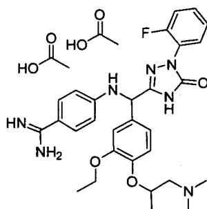
[Chemical Formula 716]
