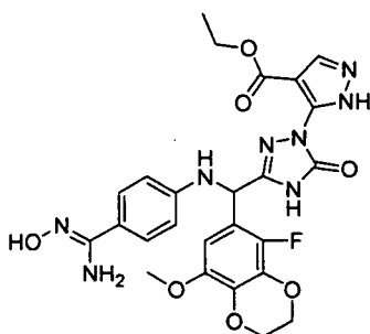
[Chemical Formula 514]
