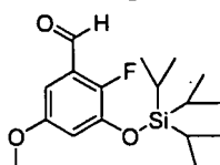
[Chemical Formula 51]
