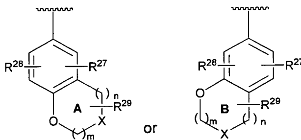
[Chemical Formula 19]
