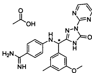
[Chemical Formula 276]
