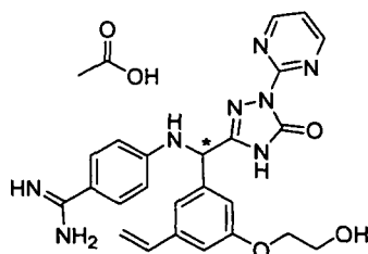
[Chemical Formula 199]
