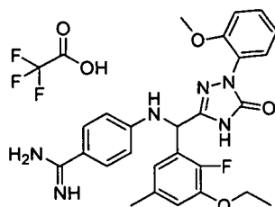
[Chemical Formula 620]
