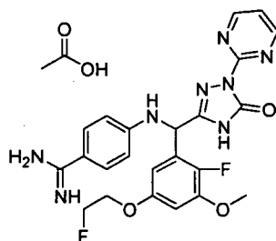
[Chemical Formula 734]
