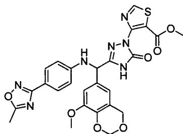
[Chemical Formula 424]
