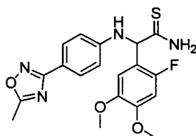
[Chemical Formula 33]
