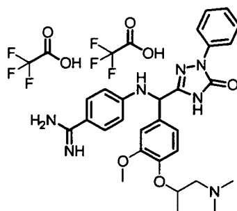
[Chemical Formula 749]
