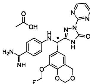
[Chemical Formula 631]
