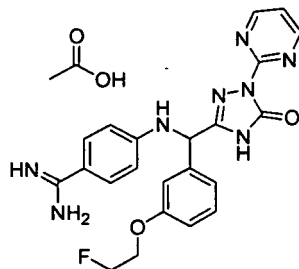
[Chemical Formula 708]
