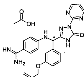
[Chemical Formula 588]
