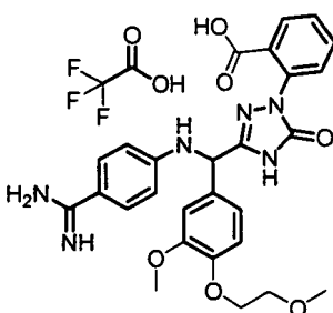
[Chemical Formula 744]
