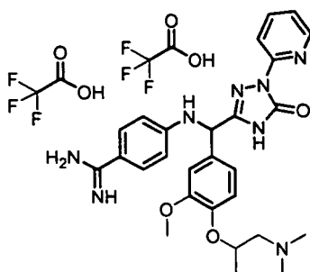
[Chemical Formula 755]
