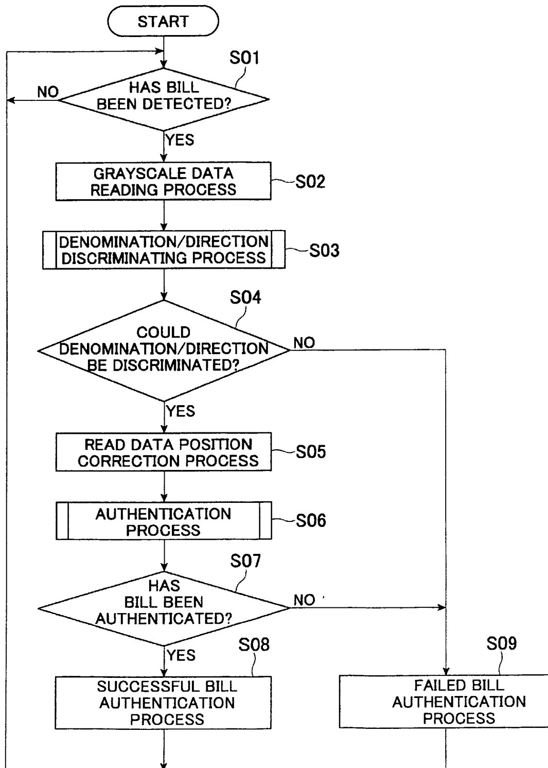
(MAIN AUTHENTICATION FLOWCHART)
