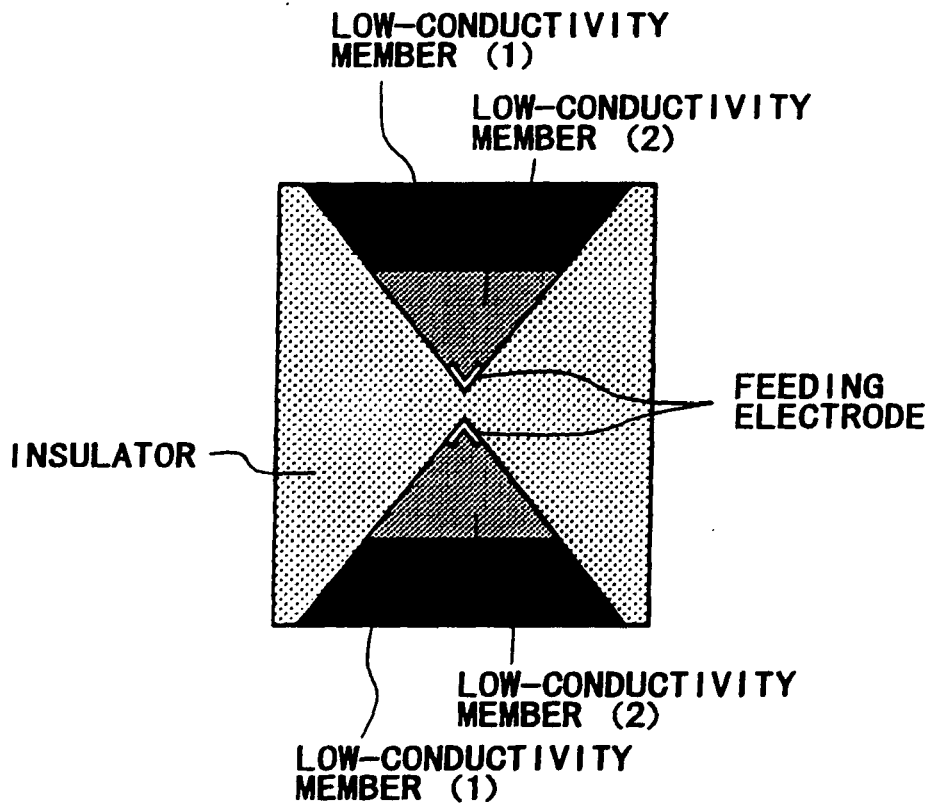
CROSS-SECTIONAL VIEW
