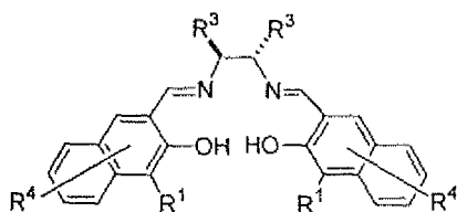
Salen Ligand (30)
