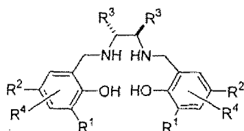
Salan Ligand (29')
