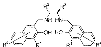
Salan Ligand (31')
