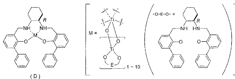
Salan Ligand (42')
