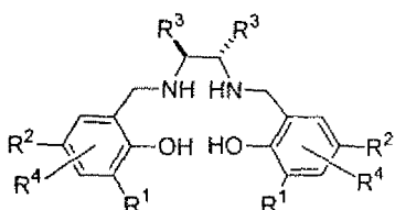
Salan Ligand (29)
