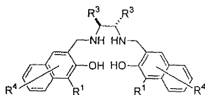
Salan Ligand (31)
