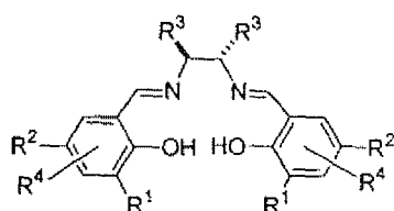
Salen Ligand (28)
