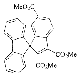
Spirodihydroindolizines
