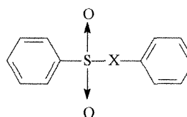
Aryl thiosulfonates
