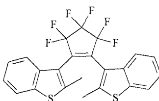
Diarylethenes
