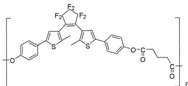
Diarylethene polymer
