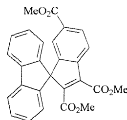
Spirodihydroindolizines
