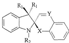
Spiropyran (X=O; Y=-CH) Spiioxazine (X=O; Y=N) Thiospiropyran (X=S; Y=CH)
