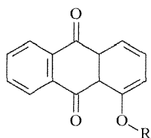
Quinone
