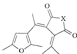
Fulgides (X=O) Fulgimides (X=NR)
