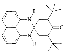
Perimidinespirocyclohexadienones
