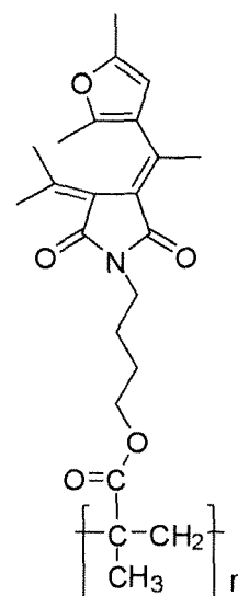
Fulgide polymer
