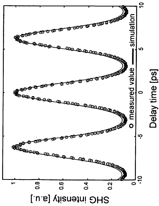
(a) Auto-correlation waveform
