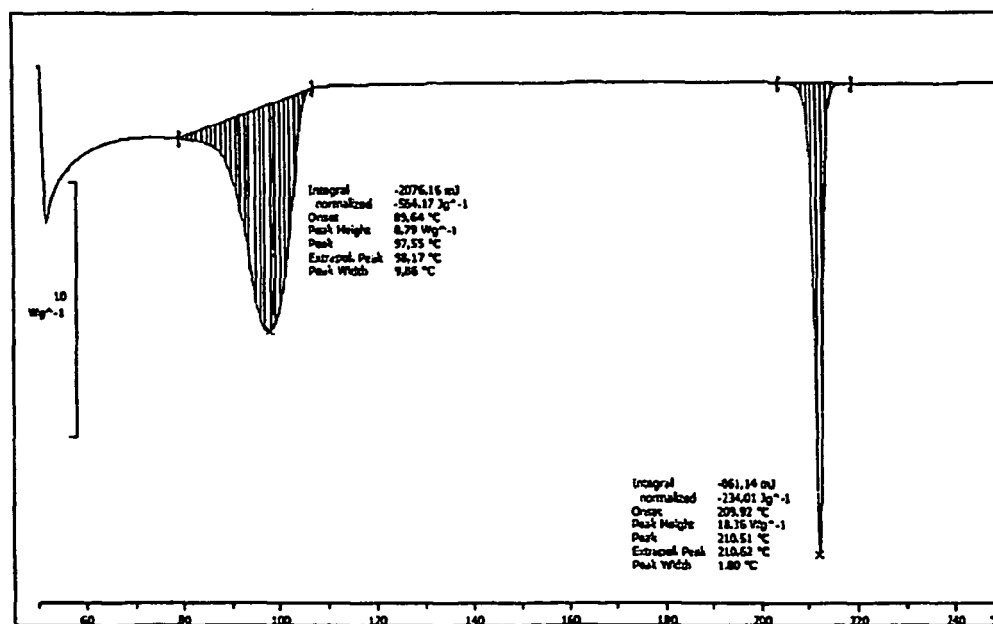
Figure 4: DSC curve of the crystalline Imatinib base of the the present invention.
