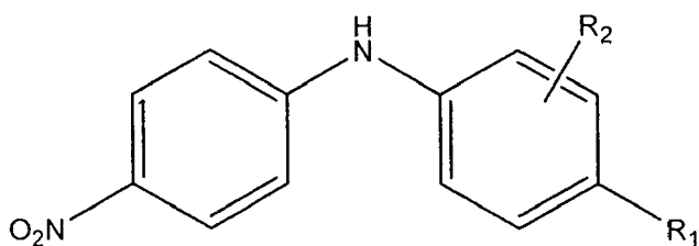
Formula I
