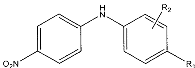
Formula I
