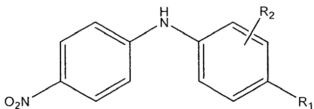
Formula I
