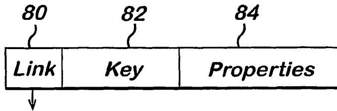
Fig. 5 Logical Structure of a Conclusion Set Entry
