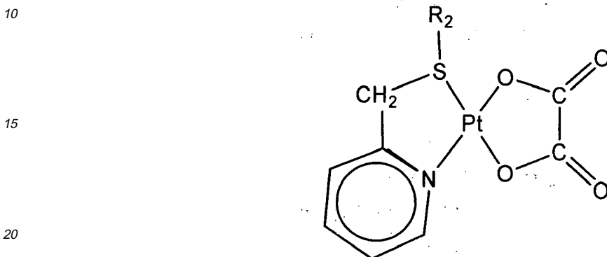
Formula (II)
