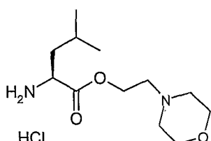
Intermediate 14
