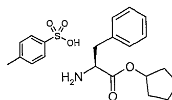
Intermediate 16
