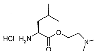
Intermediate 13
