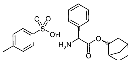
Intermediate 12
