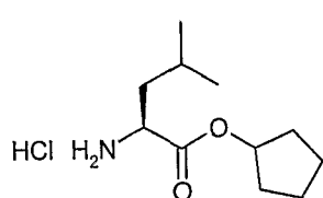
Intermediate 8
