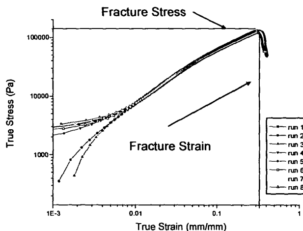
Figure 2. Typical stress-strain curve with fracture stress and fracture strain marked at the peak of the stress-strain curve. Multiple runs are shown.
