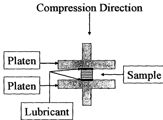
Figure 1. Experimental configuration for lubricated squeezing test
