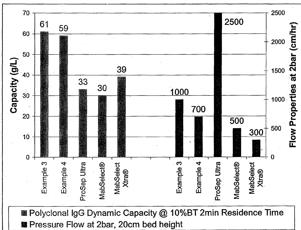
Figure 1. Comparison of Invented Method to Commercial Affinity Media
