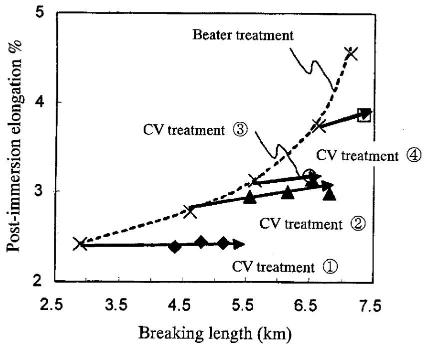
Relationship between breaking length and post-immersion elongation
