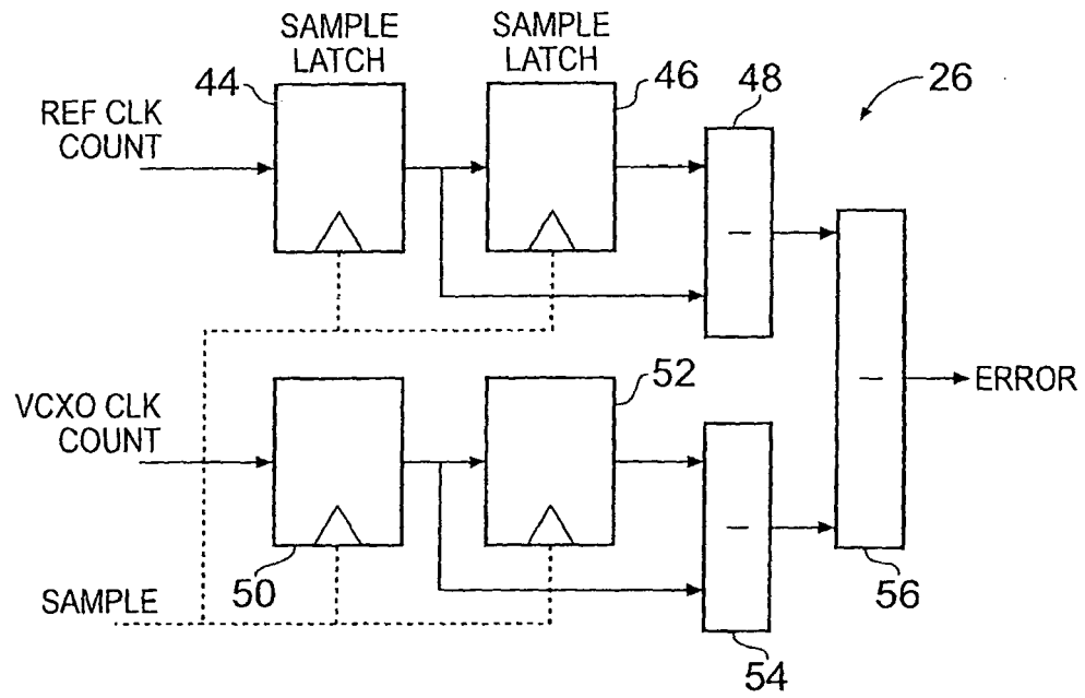
Fig. 5: Clock Difference Circuit
