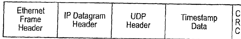
Fig. 3: UDP Timestamp Packet
