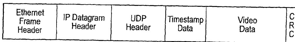
Fig. 8: Combined Packet
