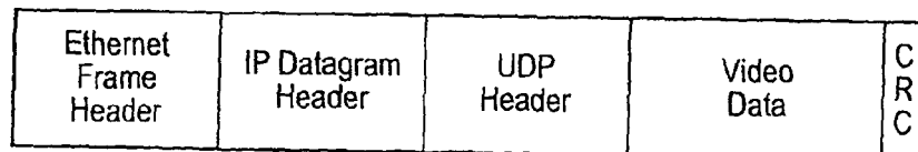
Fig. 7: Video Packet
