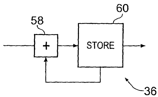
Fig. 6: Accumulator
