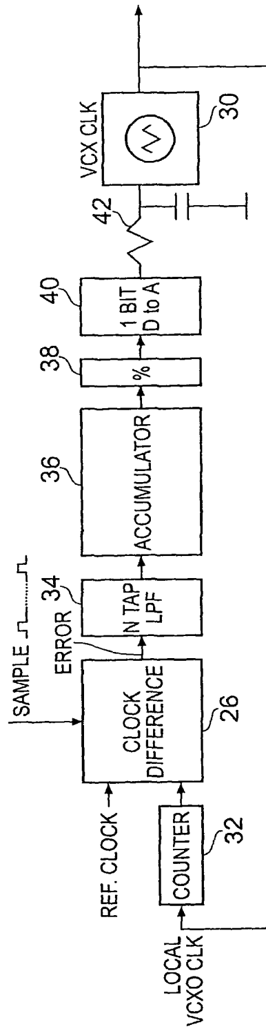
Fig. 4: Frequency Locking System
