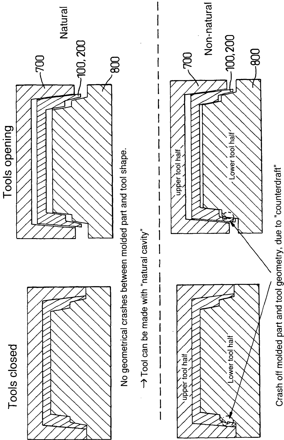
Natural and non-natural cavities Fig. 13
