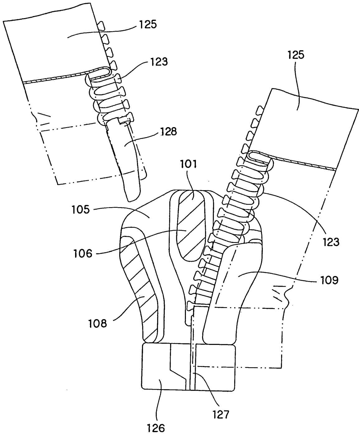
FIG. 12 PRIOR ART
