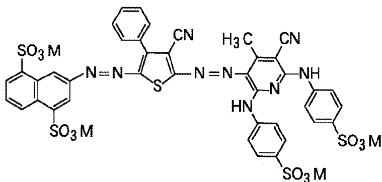
Exemplified compound VII-1
