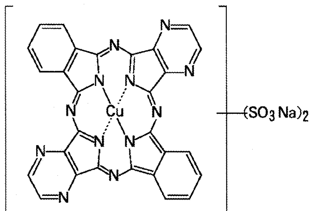
Compound (17)
