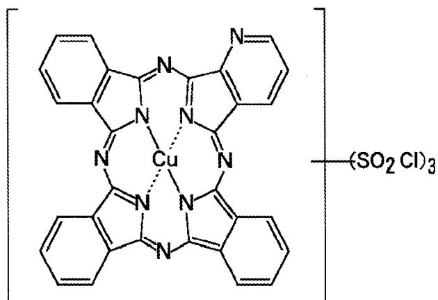
Compound (3)
