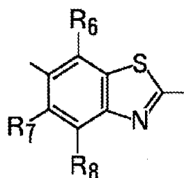
General formula (4)
