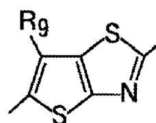
General formula (5)
