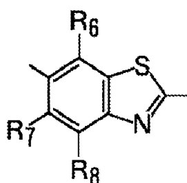
General formula (4)
