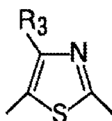
General formula (2)
