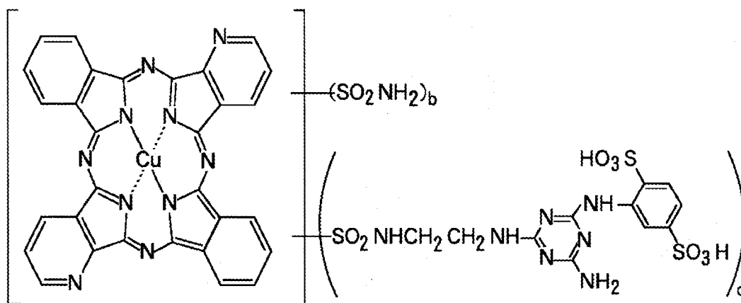
Compound (7)
