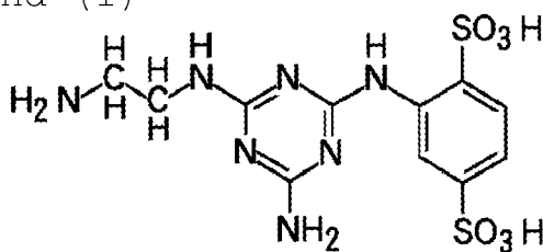
Compound (1)
