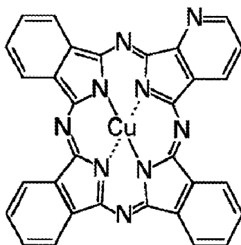
structural formulae 2
