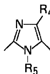
General formula (3)
