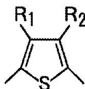
General formula (1)
