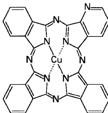
Compound (2)
