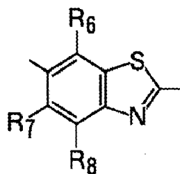
General formula (4)
