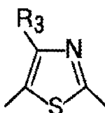
General formula (2)
