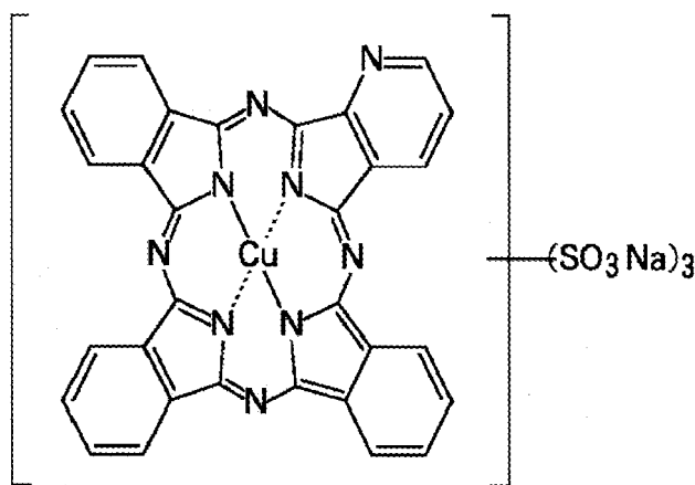
Compound (11)
