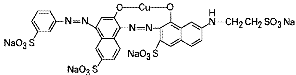
Comparative compound 5
