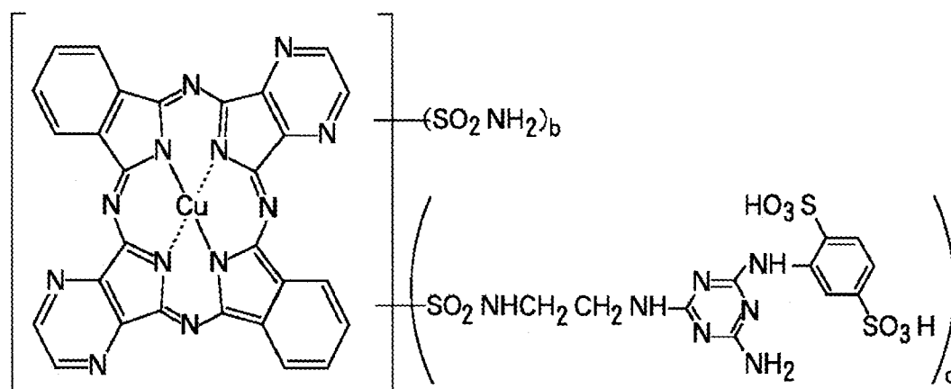
Compound (19)
