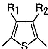
General formula (1)
