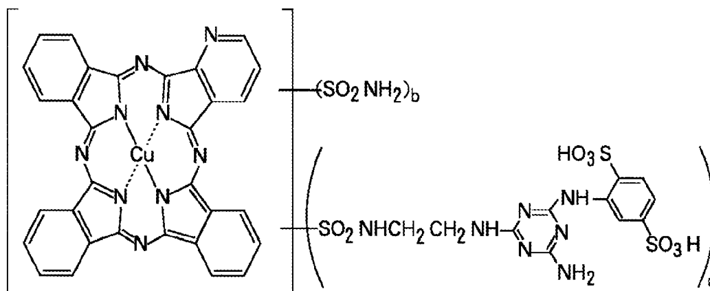
Compound (4)
