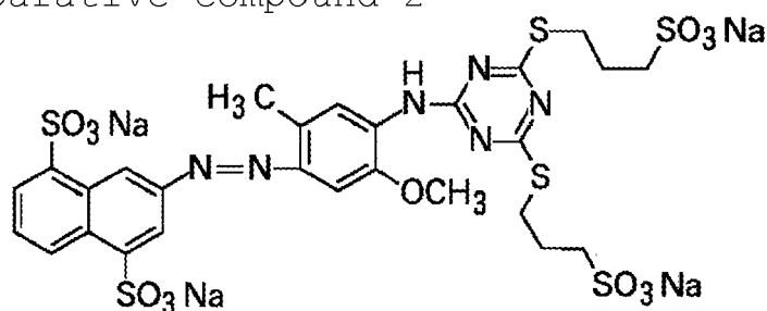
Comparative compound 2
