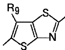
General formula (5)
