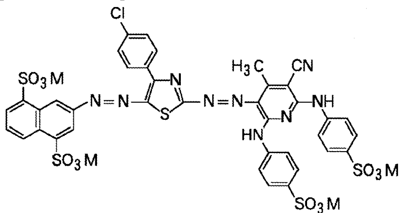
Exemplified compound VII-3
