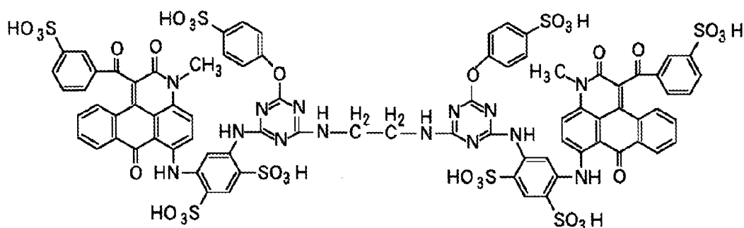
Exemplified compound III-1
