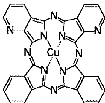
Structural formula 1C
