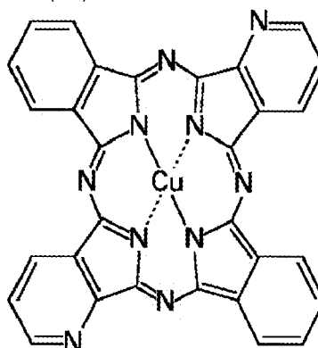
Compound (5)
