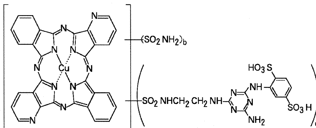
Compound (16)
