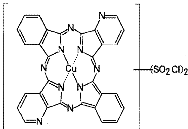
Compound (15)
