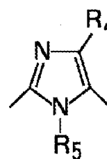
General formula (3)
