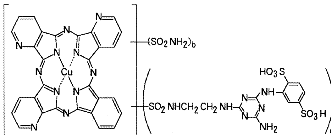
Compound (10)
