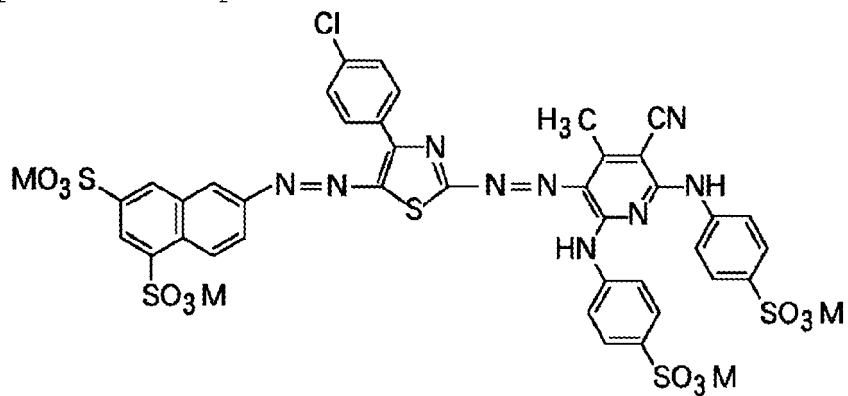
Exemplified compound VII-11
