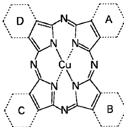
General formula (A)
