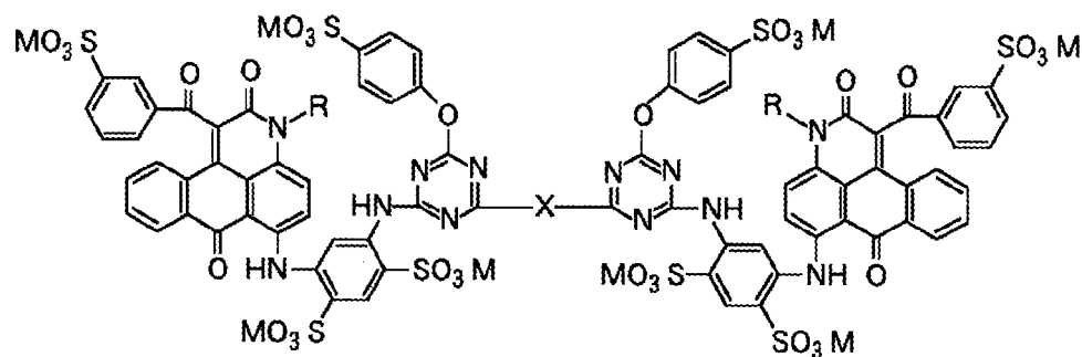
General formula (III)
