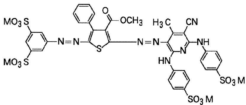
Exemplified compound VII-4
