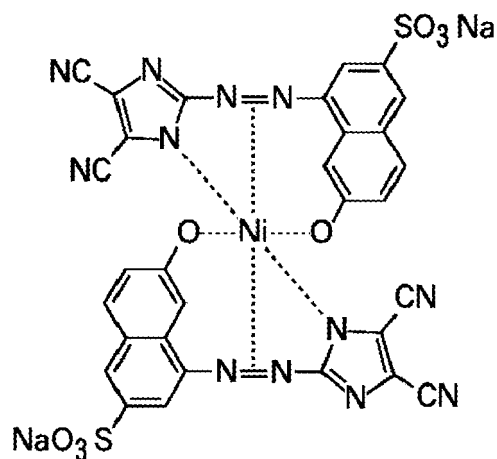
Comparative compound 3
