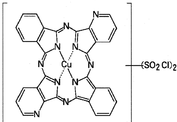
Compound (6)
