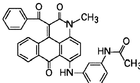
Formula (3)
