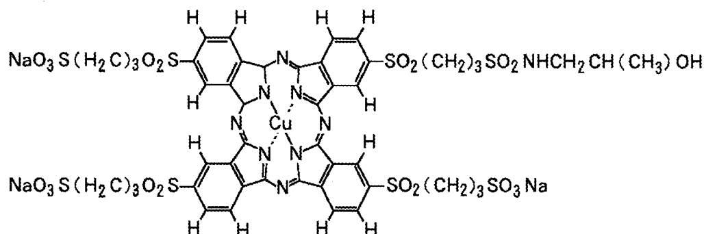
Comparative compound 1
