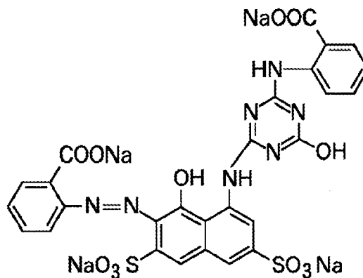
Comparative compound 4
