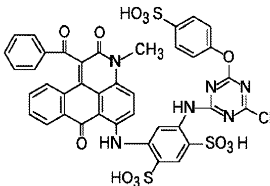
Formula (6)
