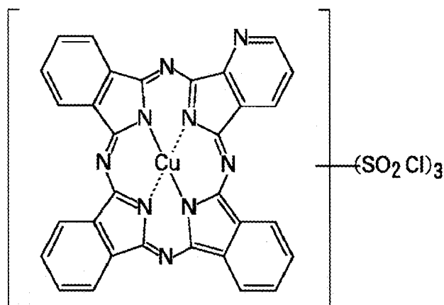
Compound (12)
