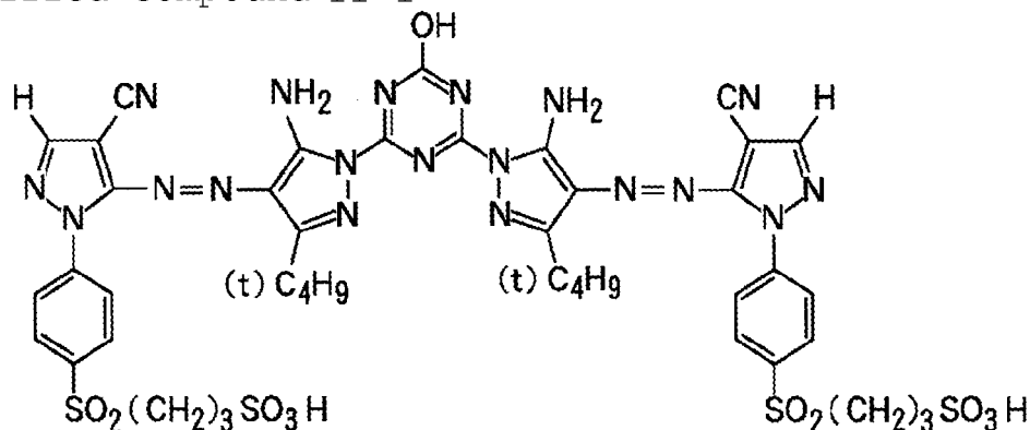
Exemplified compound II-1
