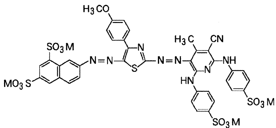
Exemplified compound VII-9
