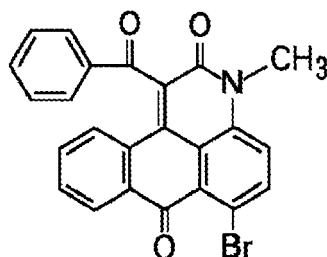
Formula (2)
