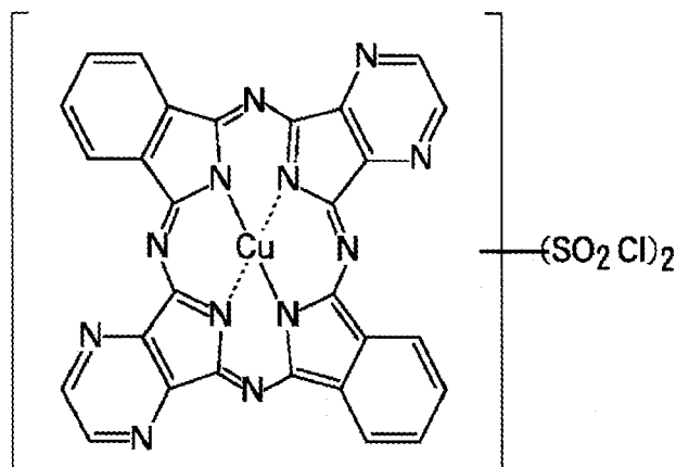
Compound (18)
