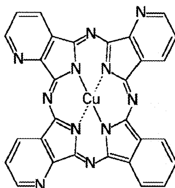
Compound (8)
