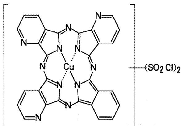
Compound (9)
