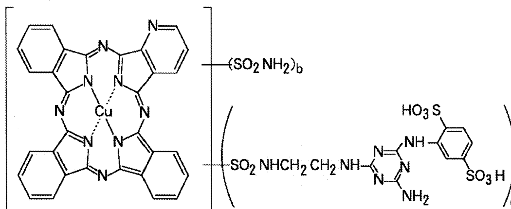
Compound (13)
