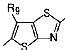
General formula (5)
