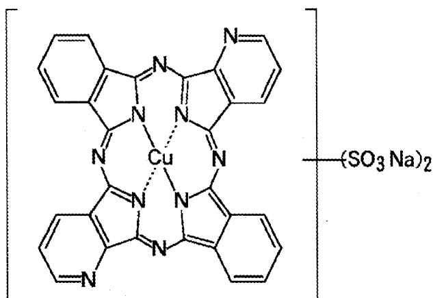
Compound (14)
