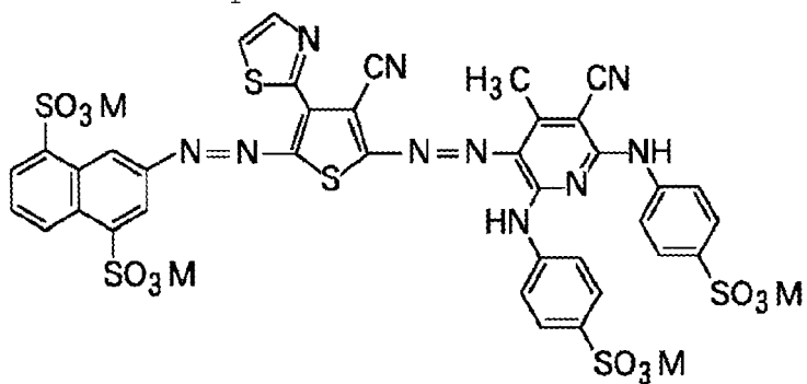
Exemplified compound VII-7
