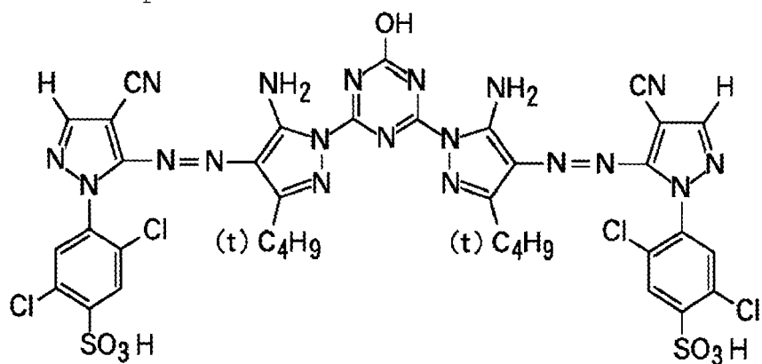
Exemplified compound II-9
