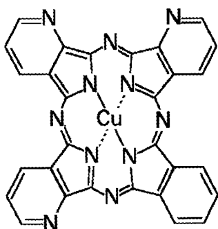
Structural formulae 3C
