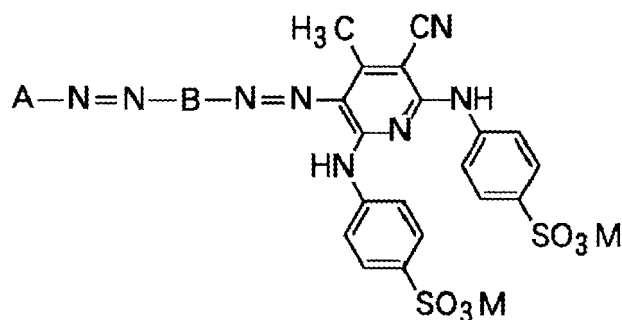
General formula (VII)
