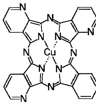
Structural formulae 3B
