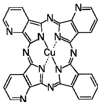
Structural formulae 3A
