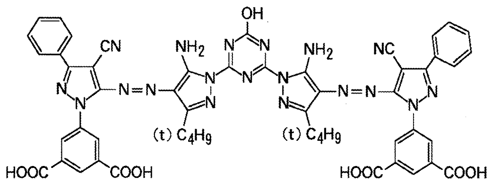
Exemplified compound II-8
