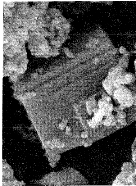
MgO PARTICLE FORMED BY GAS-PHASE METHOD
