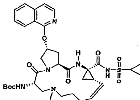
15 20 25 Compound 147
