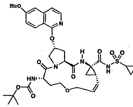
compound 141
