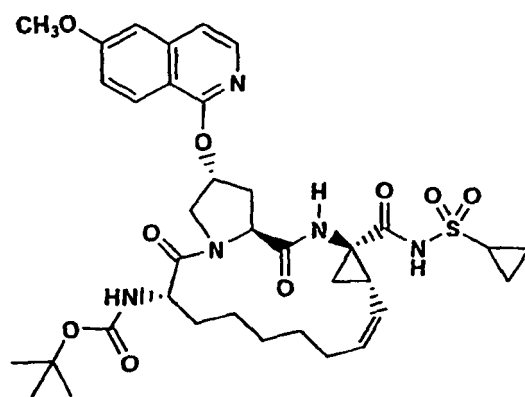
Compound 17B
