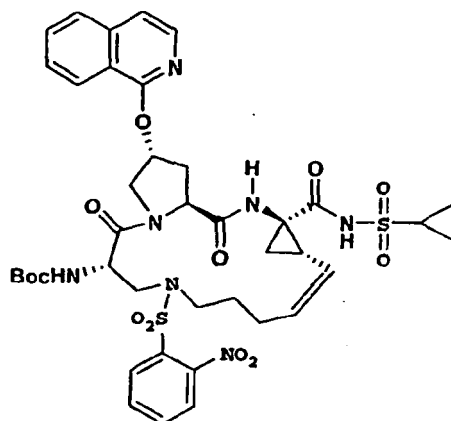
compound 145
