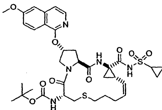
Compound 18B
