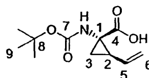
1S,2R-acid
