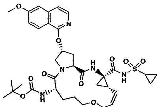
Compound 28
