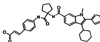
Replicase Inhibitor Compound Y, WO 03/010141
