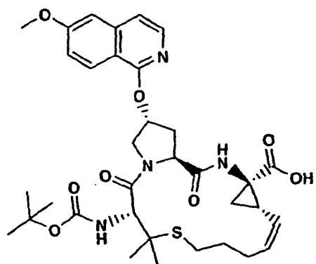
Compound 79
