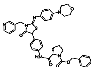
NS5A Inhibitor
