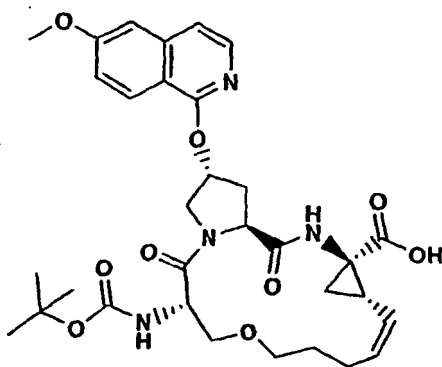
Compound 84
