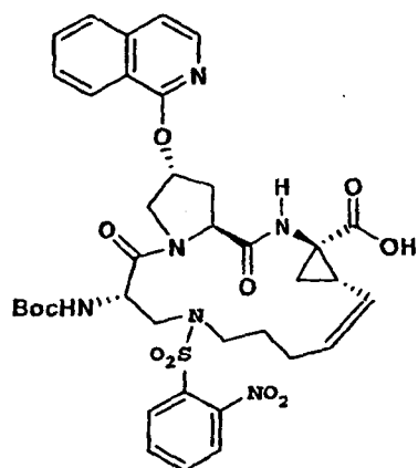
Compound 144
