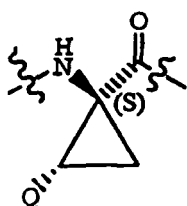
Q syn to carbonyl
