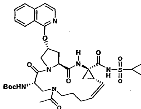
Compound 146
