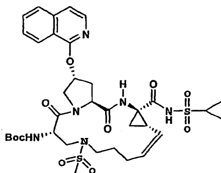
Compound 153
