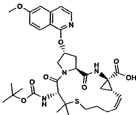
Compound 79
