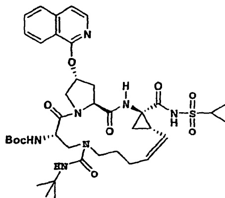
Compound 150
