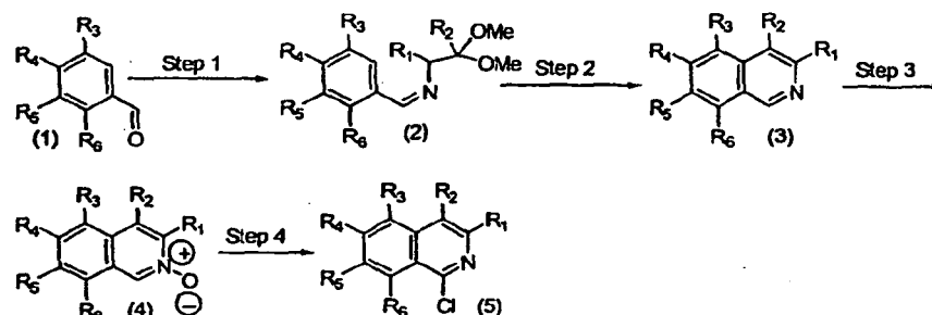
Pomeranz-Fritsch synthesis K. Hirao, R. Tsuchiya, Y. Yano, H. Tsue, Heterocycles 42(1) 1996, 415-422
