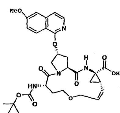
compound 140
