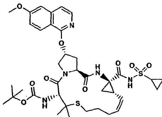
Compound 80
