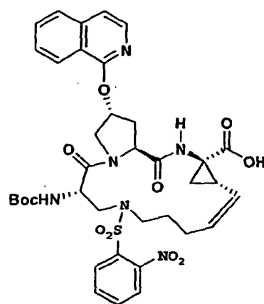
compound 144
