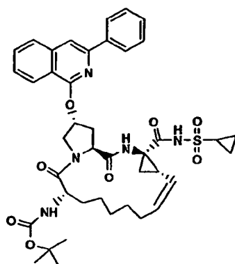
compound 58
