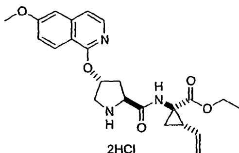
Example 22
