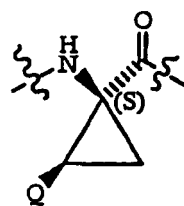
Q syn to nitrogen
