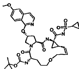
Protease Inhibitor Compound 28
