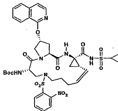
Compound 145
