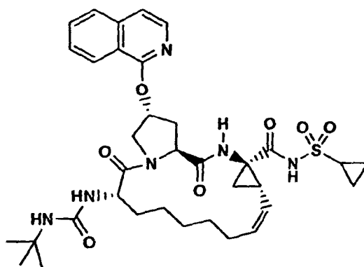
compound 126
