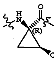
Q syn to nitrogen
