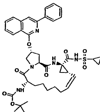
compound 58
