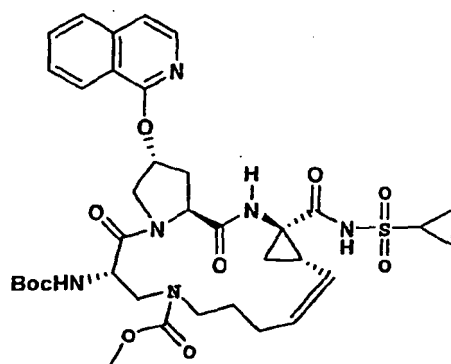
Compound 148
