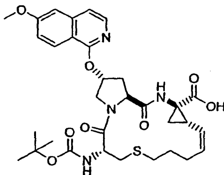
Compound 18A
