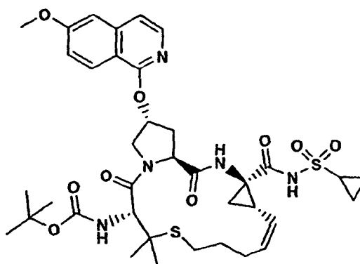
Compound 80
