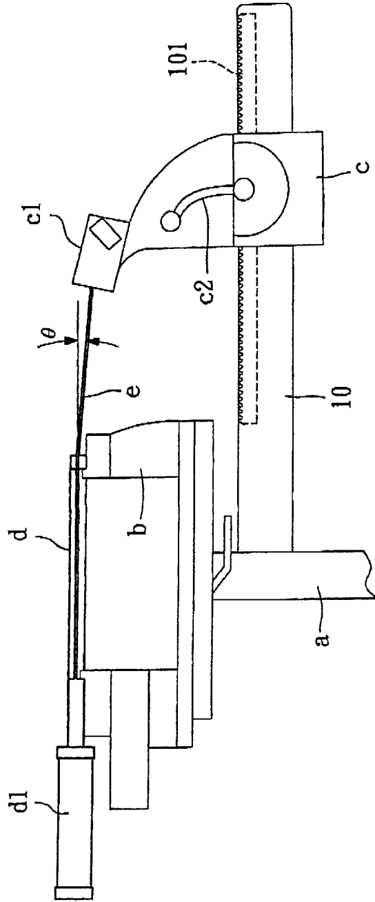
FIG. 2 PRIOR ART
