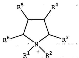
PYRROLIDINIUM
