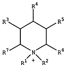
PIPERIDINIUM
