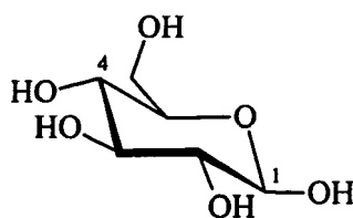
\beta -D-glucose
