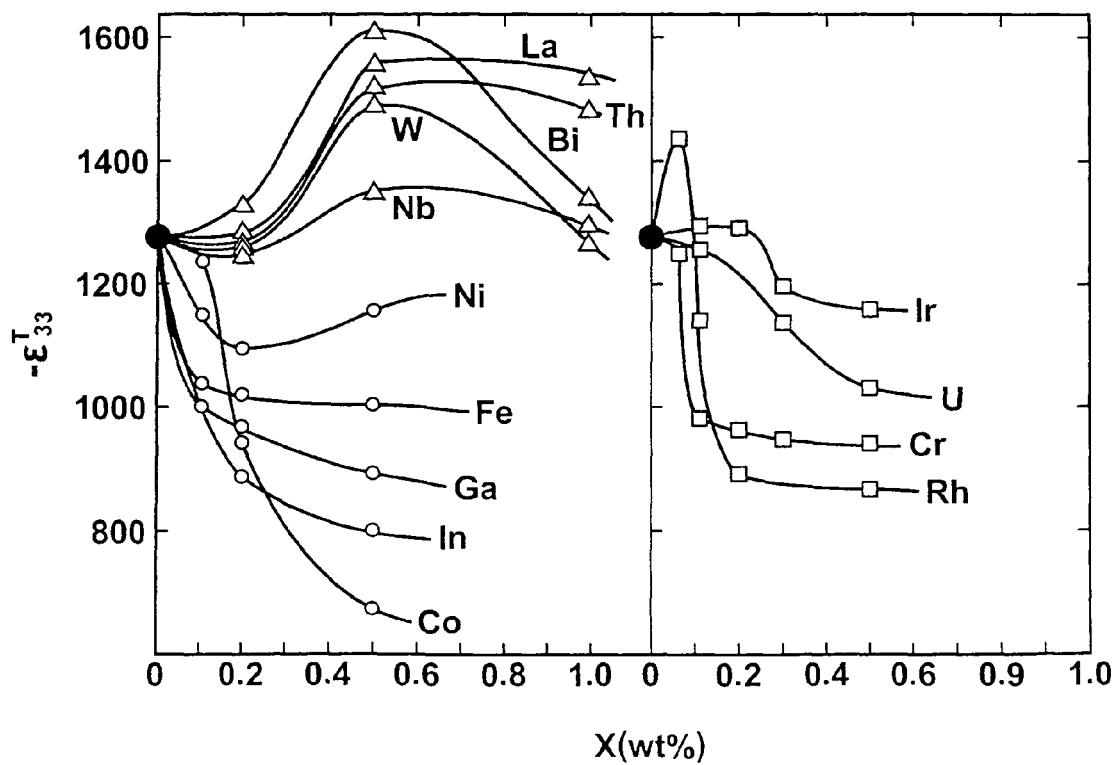
FIG.10 PRIOR ART
