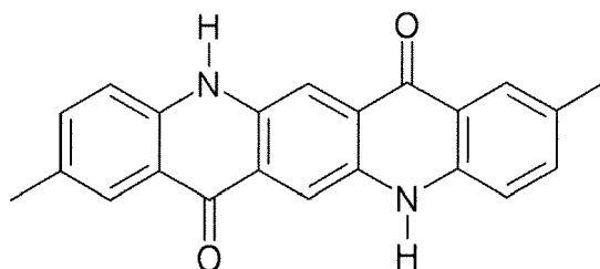
Pigment PR 122 (2,9-dimethylquinacridone)
