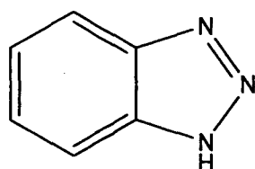
[Chem. 47]
