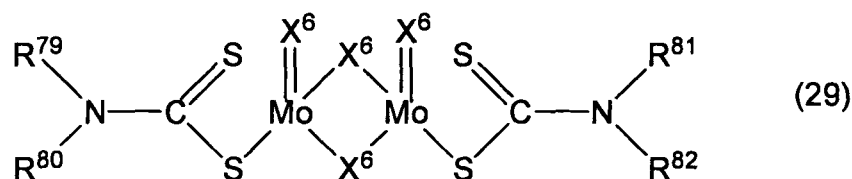
[Chem. 35]
