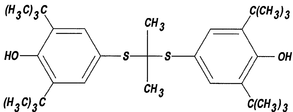
Probucol
