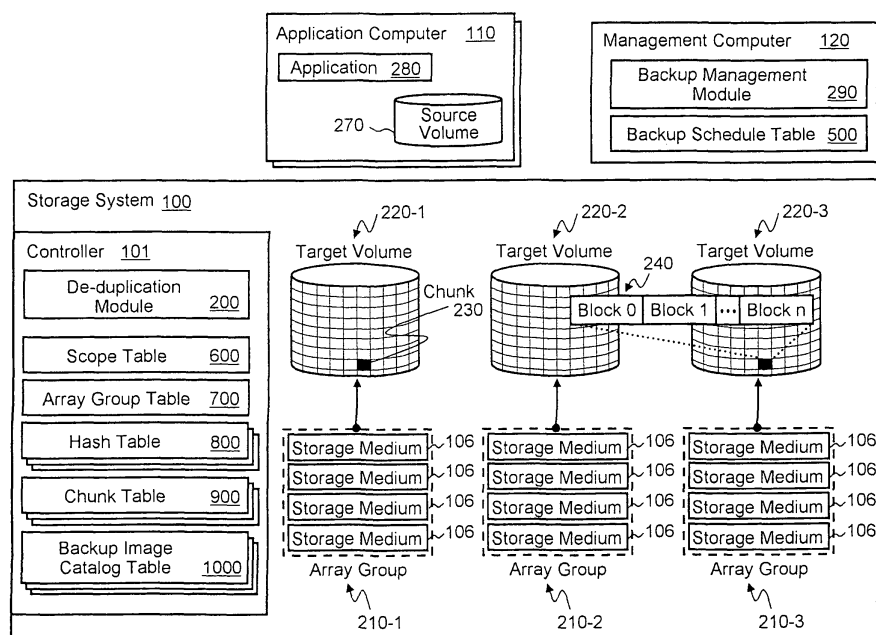
FIG. 2 Logical Element Structure
