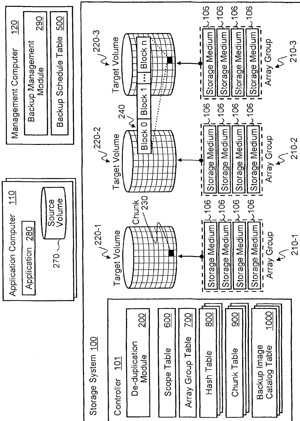
FIG. 2 Logical Element Structure
