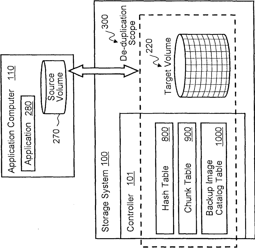
FIG. 3 Logical Structure of De-duplication Scope
