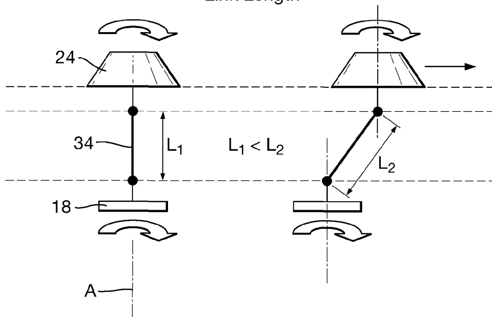
Fig.2. Link Length
