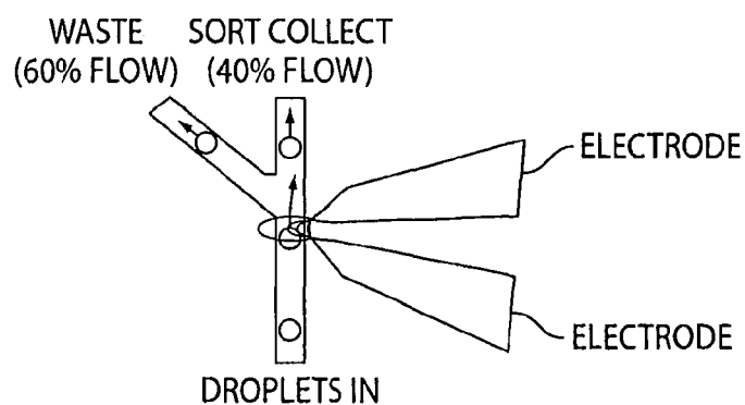
FLIPPED FLUIDIC GEOMETRY (ASYMMETRIC FLOW GEOMETRY)
