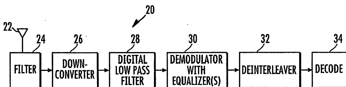
FIG. 1 (PRIOR ART)
