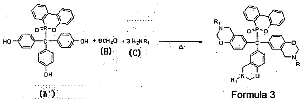
&lt;Reaction Scheme 2&gt;
