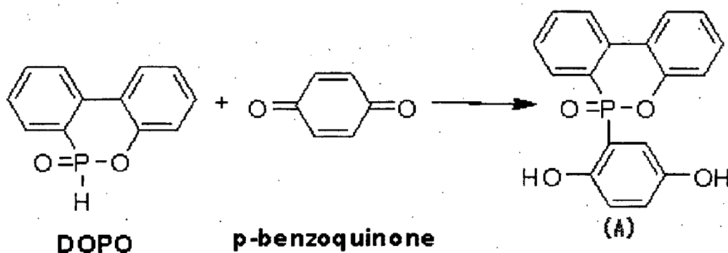
<Reaction Scheme 3>
