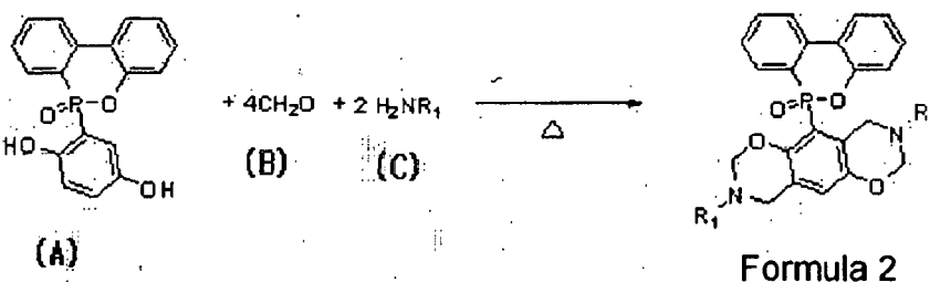
&lt;Reaction Scheme 2&gt;
