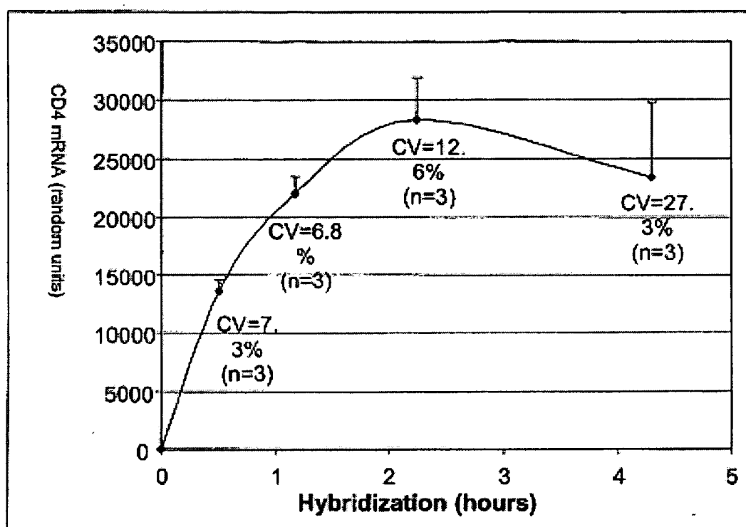
FIG 9. Hybridization kinetics
