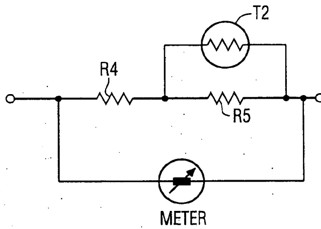
FIG. 3 PRIOR ART
