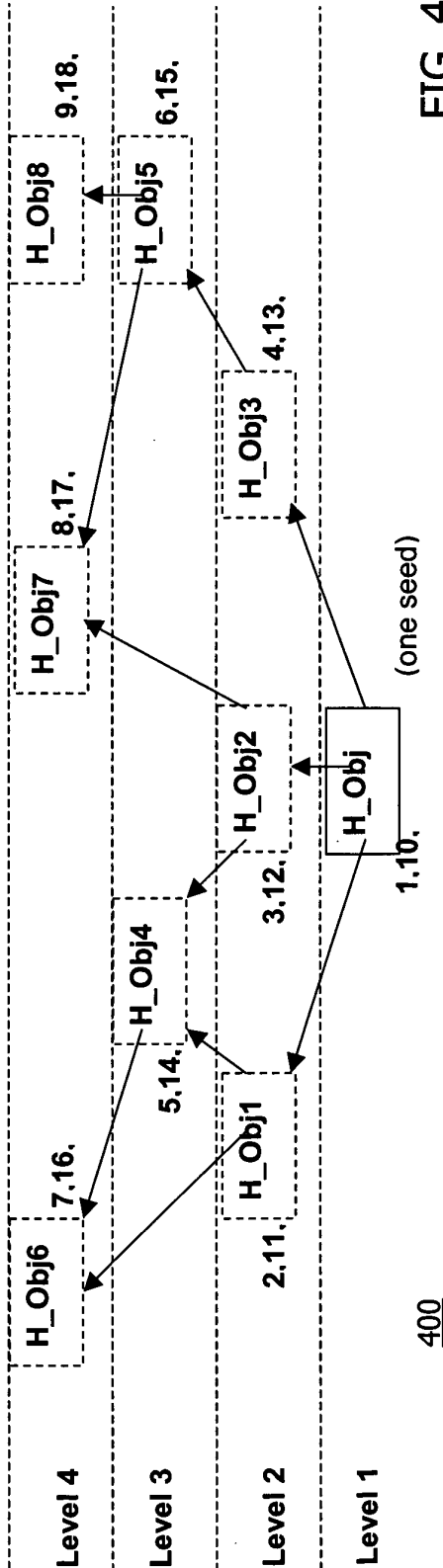
Breadth-First-Search
