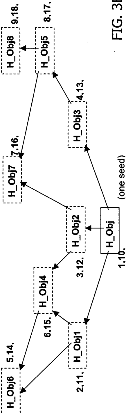
Breadth-First-Search
