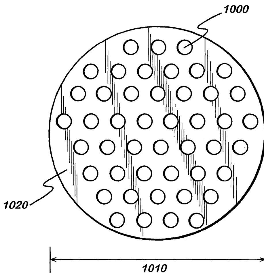
Fig. 3 Distillation Tray
