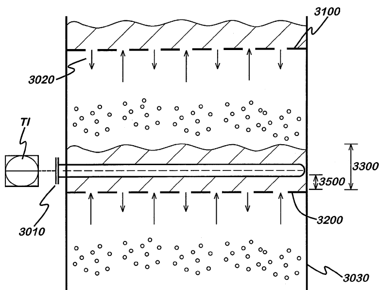
Fig. 5 Temperature control
