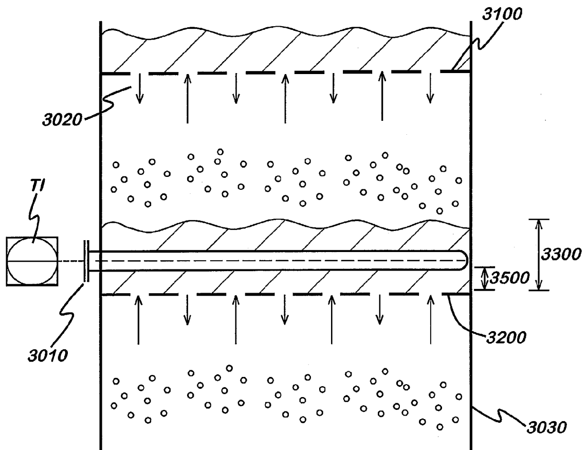
Fig. 5 Temperature control
