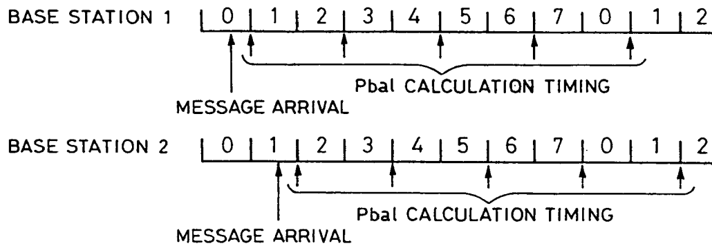
CONVENTIONAL PbaI CALCULATION TIMING (Nperiod=2)
