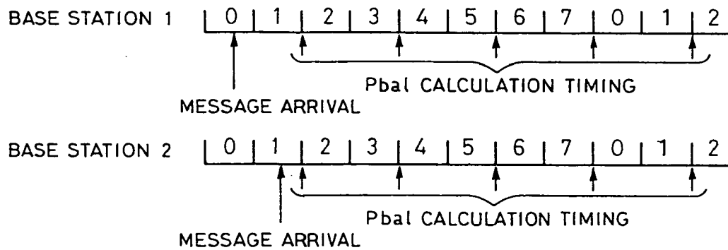
PbaI CALCULATION TIMING OF PRESENT INVENTION (Nperiod=2)
