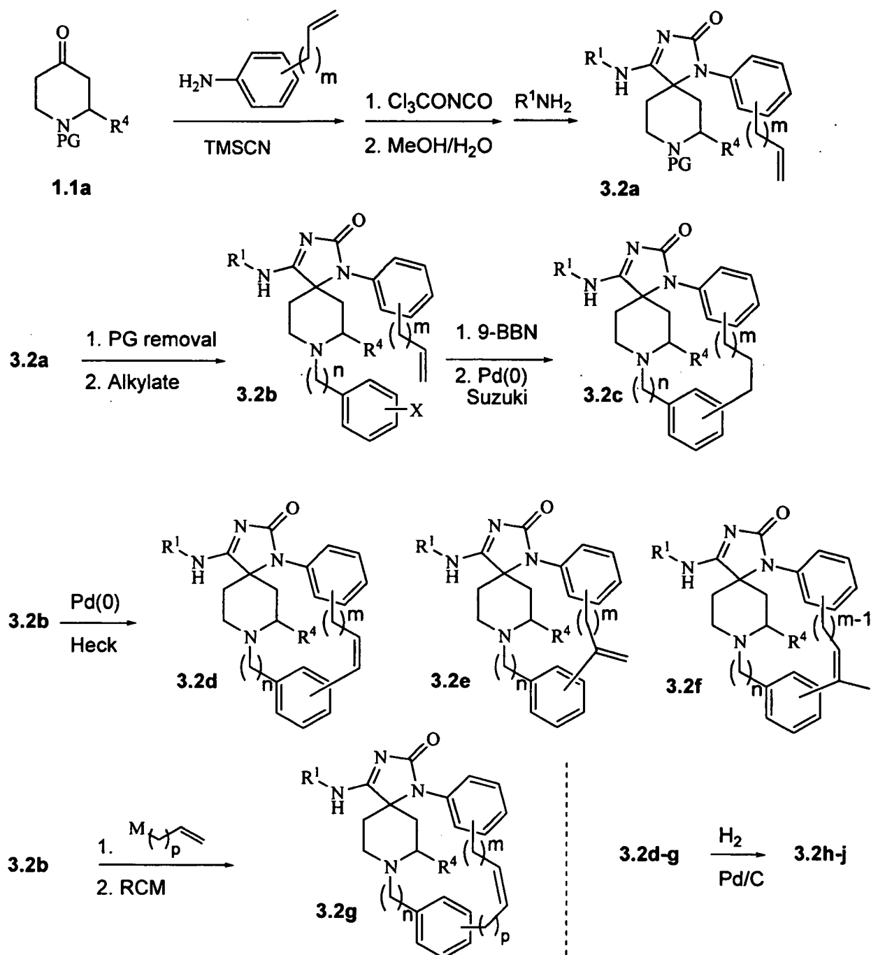
Scheme 3.2
