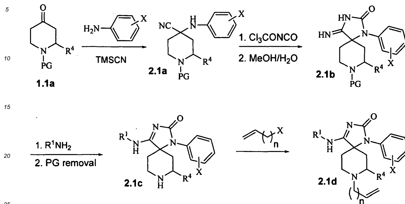
Scheme 2.1
