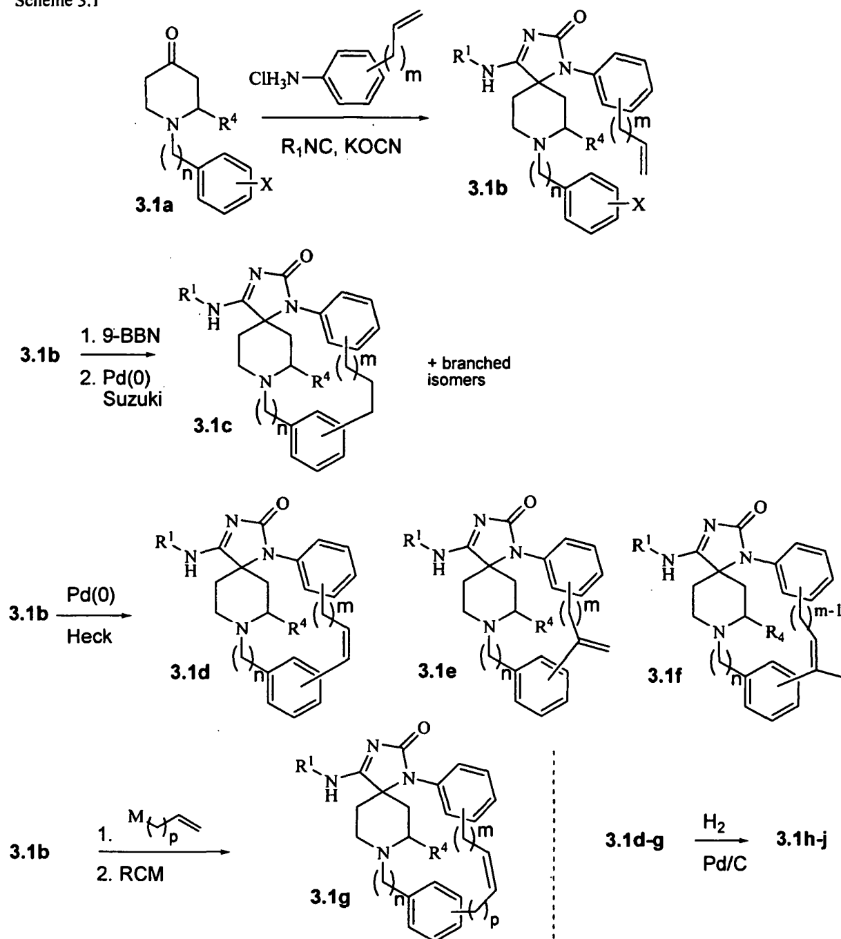
Scheme 3.1
