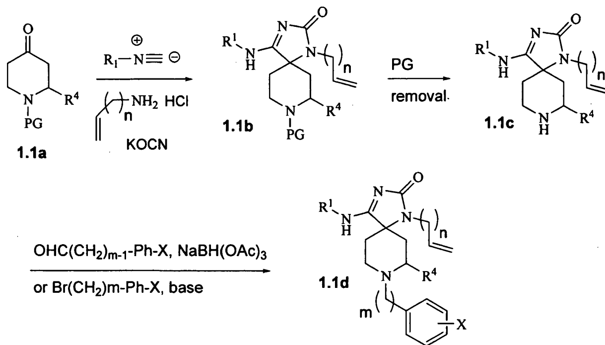
Scheme 1.1
