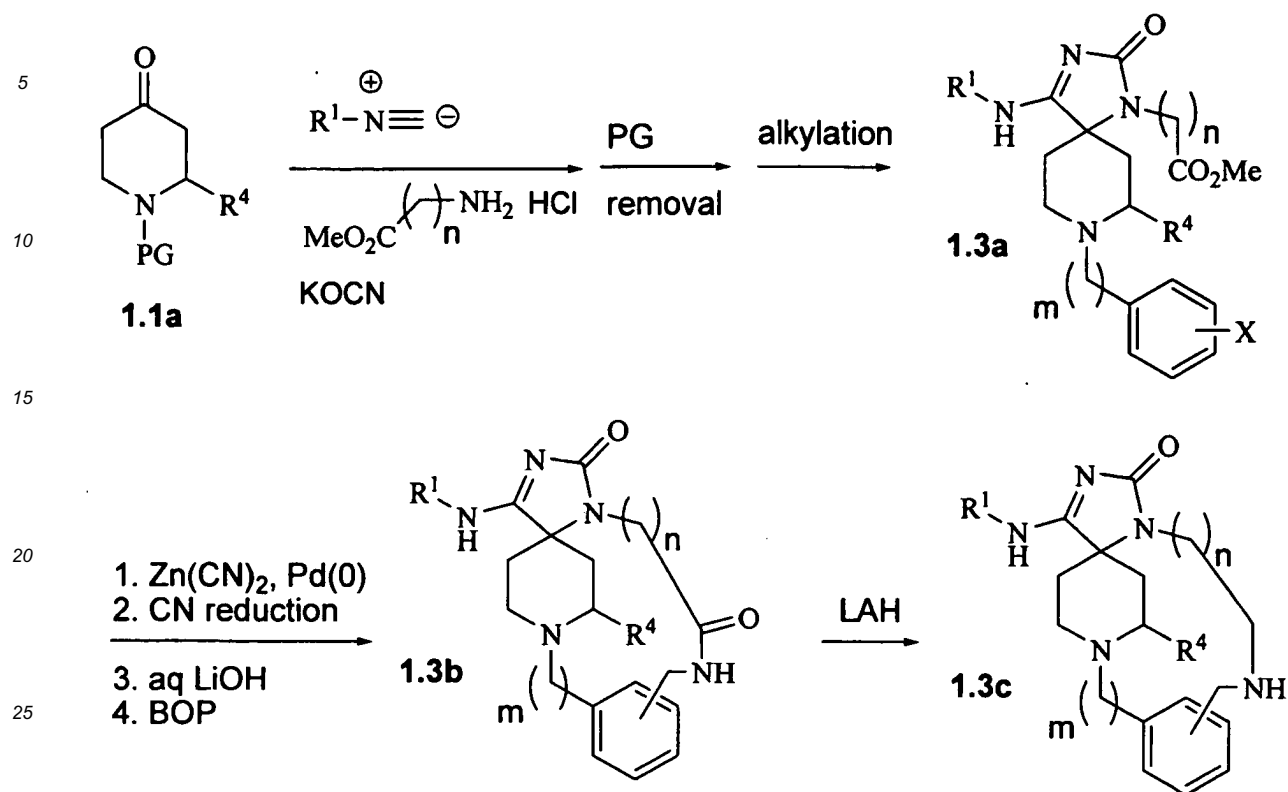
Scheme 1.3
