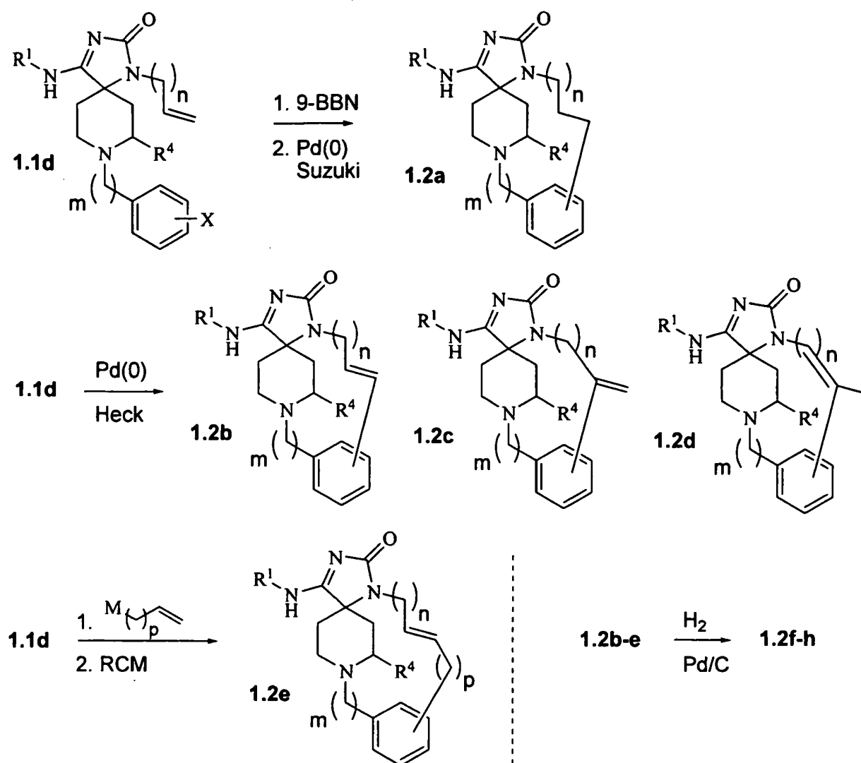
Scheme 1.2
