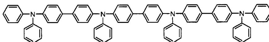
[Chemical Formula 11]
