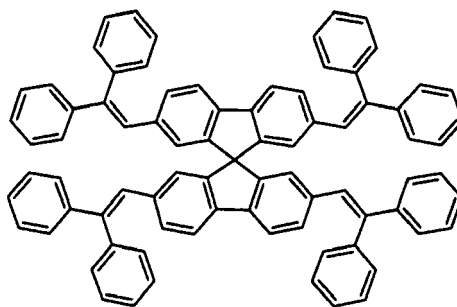
[Chemical Formula 16]
