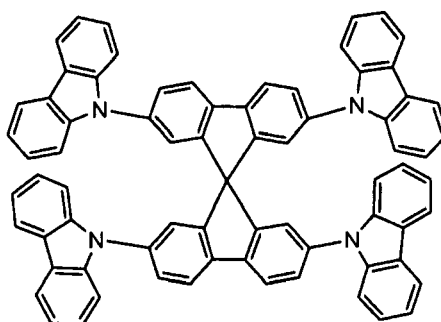
[Chemical Formula 23]
