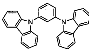
[Chemical Formula 25]
