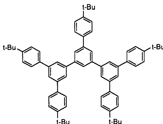
[Chemical Formula 19]
