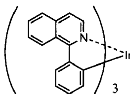
[Chemical Formula 30]
