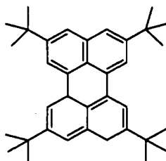
[Chemical Formula 3]
