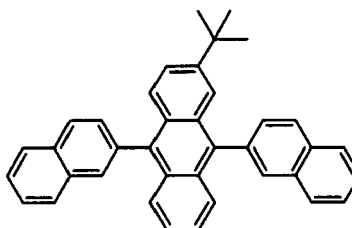
[Chemical Formula 26]
