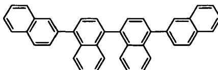
[Chemical Formula 5]
