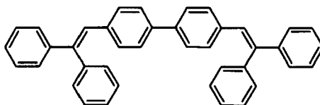
[Chemical Formula 21]
