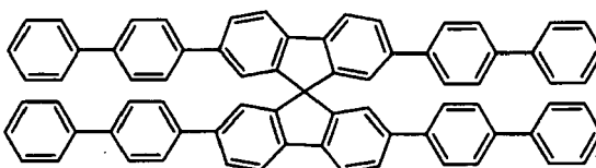
[Chemical Formula 22]
