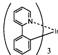
[Chemical Formula 29]
