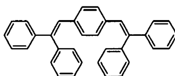
[Chemical Formula 15]
