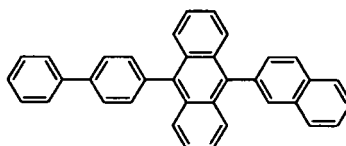
[Chemical Formula 1]
