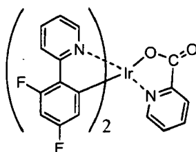
[Chemical Formula 28]
