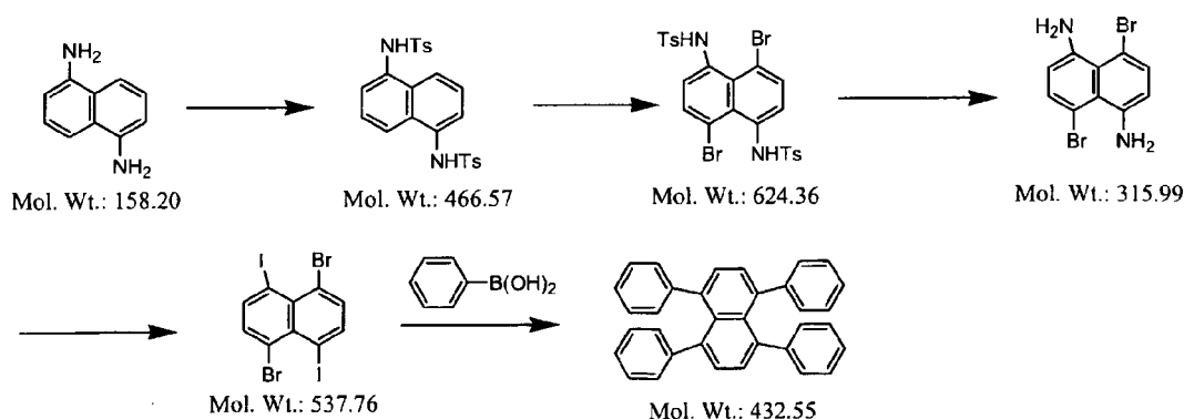
[Chemical Formula 31]
