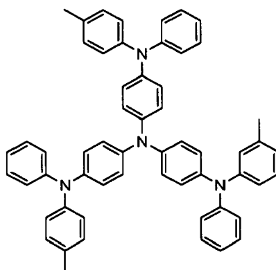
[Chemical Formula 12]
