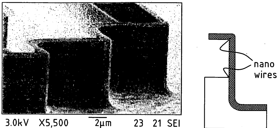
Silicon oxide mold, note the overhanging "roof".
